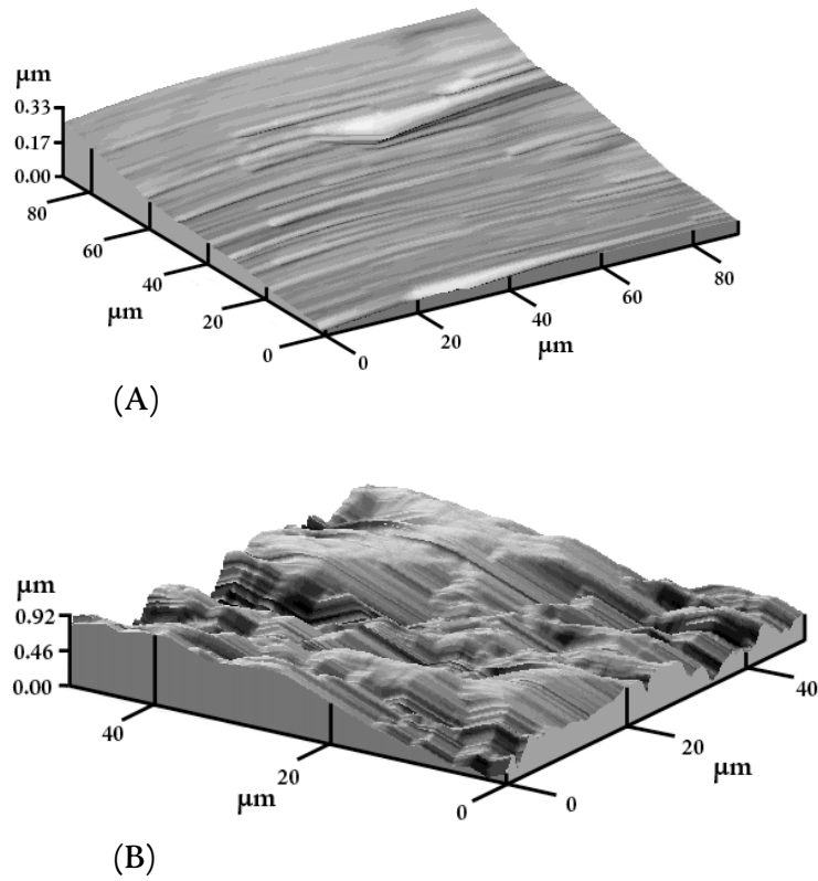
FIGURE 3: AFM images showing regions on the surfaces of (A) polished \text{Al}_2\text{O}_3 and (B) unpolished \text{Al}_2\text{O}_3 . The average roughness of the polished and unpolished surfaces is, respectively, 28 nm and 154 nm.
