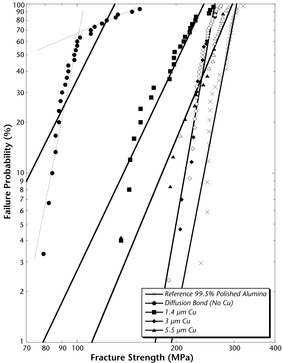
FIGURE 1: Failure probability versus fracture strength for joints processed with polished \text{Al}_2\text{O}_3 substrates. Filled symbols indicate failure along the \text{Al}_2\text{O}_3 -Nb interface; open symbols indicate failure in the ceramic.
