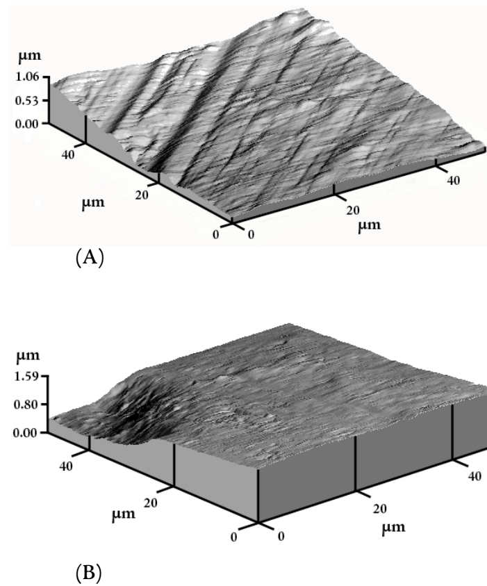
FIGURE 2: AFM images showing regions on the surfaces of (A) as-received Nb and (B) flattened Nb. Note the depression on the surface of the flattened Nb. The average roughness of the as-received and flattened Nb is, respectively, 107 nm and 97 nm.
