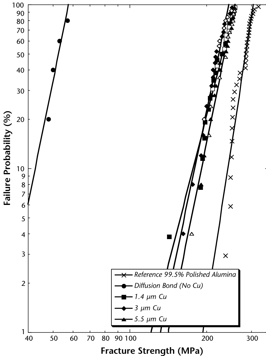
FIGURE 4: Failure probability versus fracture strength for joints processed with unpolished \text{Al}_2\text{O}_3 substrates. Filled symbols indicate failure along the \text{Al}_2\text{O}_3 -Nb interface; open symbols indicate failure in the ceramic.
