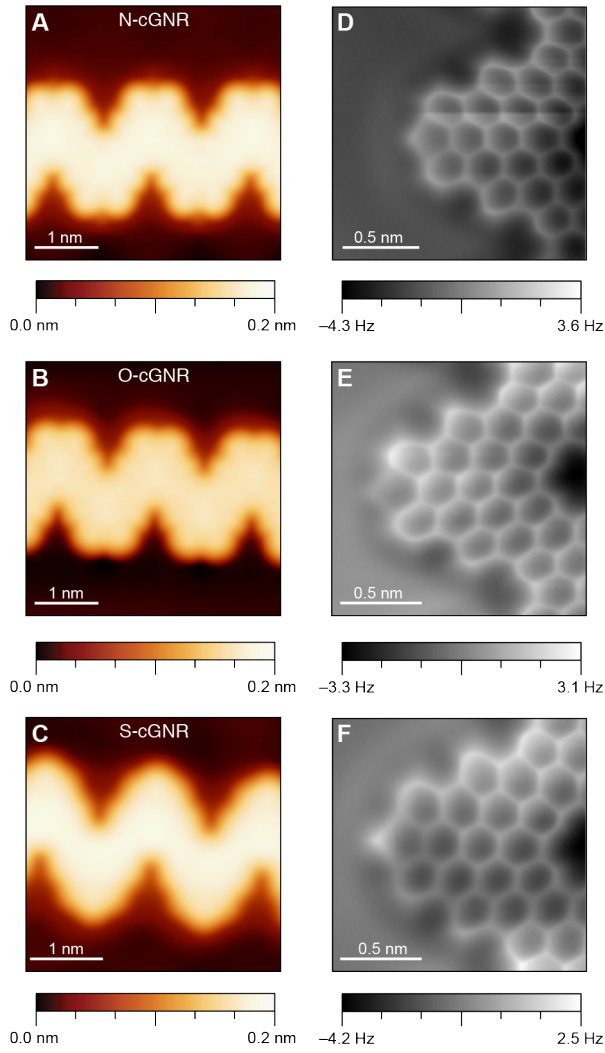
Figure 2. STM topographic image, and nc-AFM frequency shift image of (A, D) N-doped cGNRs ( V_{\text{bias}} = 10 mV, I_t = 40 pA), (B, E) O-doped cGNRs ( V_{\text{bias}} = -1.1 V, I_t = 500 pA), (C, F) S-doped cGNRs ( V_{\text{bias}} = -0.75 V, I_t = 300 pA).
