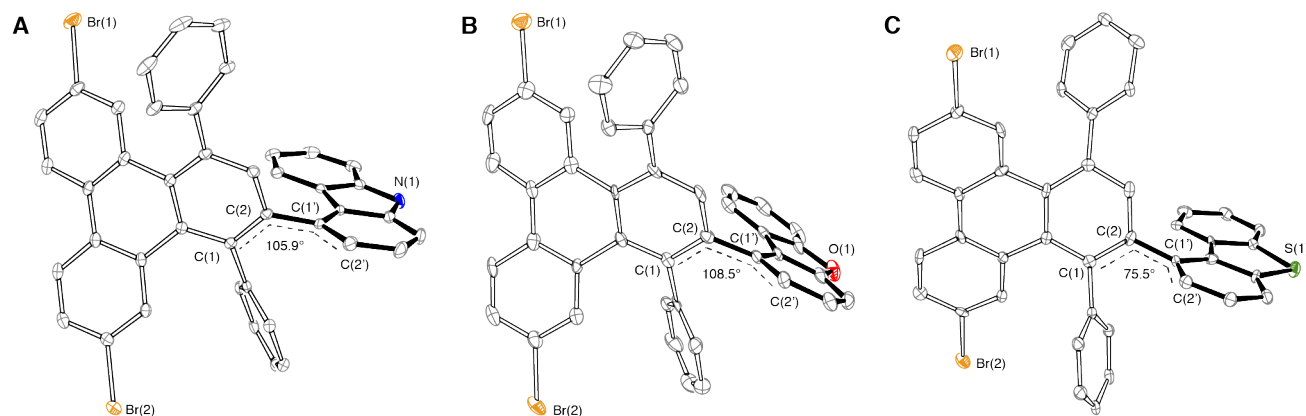
Figure 1. ORTEP representation of the molecular structures of the S_s atropisomers of (A) 1a , (B) 1b and (C) 1c found in the crystal structure. Thermal ellipsoids are drawn at the 50% probability level. Color coding: C (gray), Br (orange), N (blue), O (red), S (green). Hydrogen atoms, and solvent molecules are omitted for clarity.
