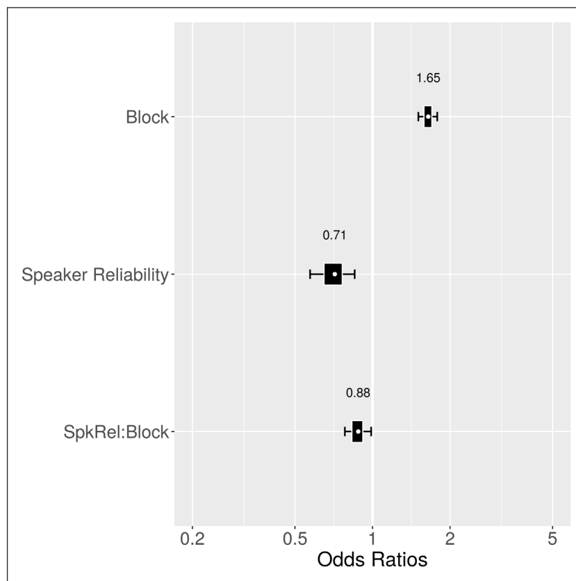
Figure 8: Odds ratio for each of the fixed effects of the first generalized mixed effects model. Solid bars indicate the posterior distribution of coefficient values for each parameter; white dots the point estimates (median); and black lines the 95% Credible Interval. SpkRel:Block = interaction between Speaker Reliability and Block.
