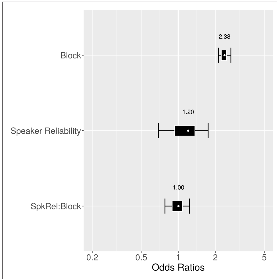
Figure 4: Odds ratio for each of the fixed effects of the first generalized mixed effects model. Solid bars indicate the posterior distribution of coefficient values for each parameter; white dots the point estimates (median); and black lines the 95% Credible Interval. SpkRel:Block = interaction between Speaker Reliability and Block
