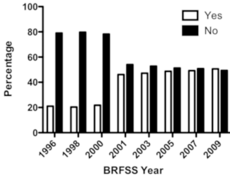
Figure 1 –. Percentage of surveyed BRFSS adults with 30+ minutes of physical activity five or more days/week (1996–2000) OR percentage with 30+ minutes of physical activity or 20+ minutes of vigorous activity five or more days/week.
