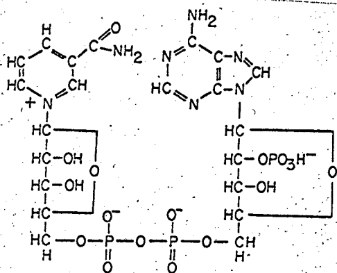
Nicotinamide adenine dinucleotide phosphate (oxidized form) (NADP + )
