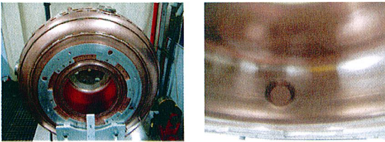
Figure 4: The cavity surface finishing after EP.
