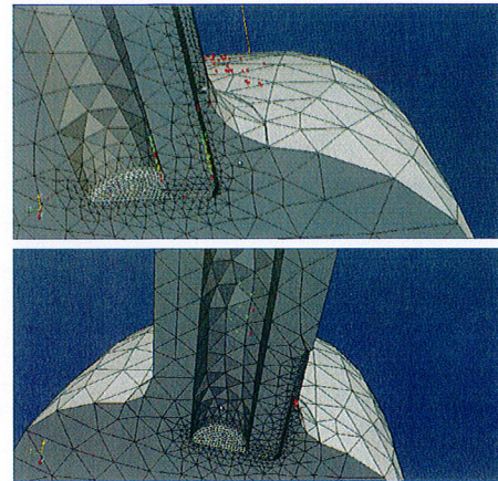
Figure 9: The impacting location of multipacting near the coupling region. The upper and lower figures are without and with external B field, respectively. The red dots are for the impacting energy between 100 to 1000 eV and the green dots are for 1000 to 2000 eV.
