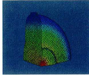
Figure 5: The cavity RF calculation in ACE3P
