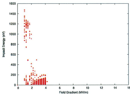
Figure 7: The multipacting spectrum near the coupling region, without external magnetic field.
