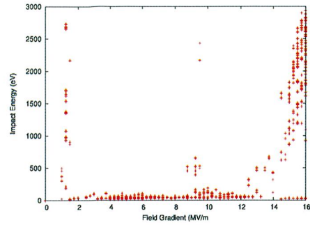
Figure 8: The multipacting spectrum near the coupling region, with external B field B = (0, 1T, 1T) .
