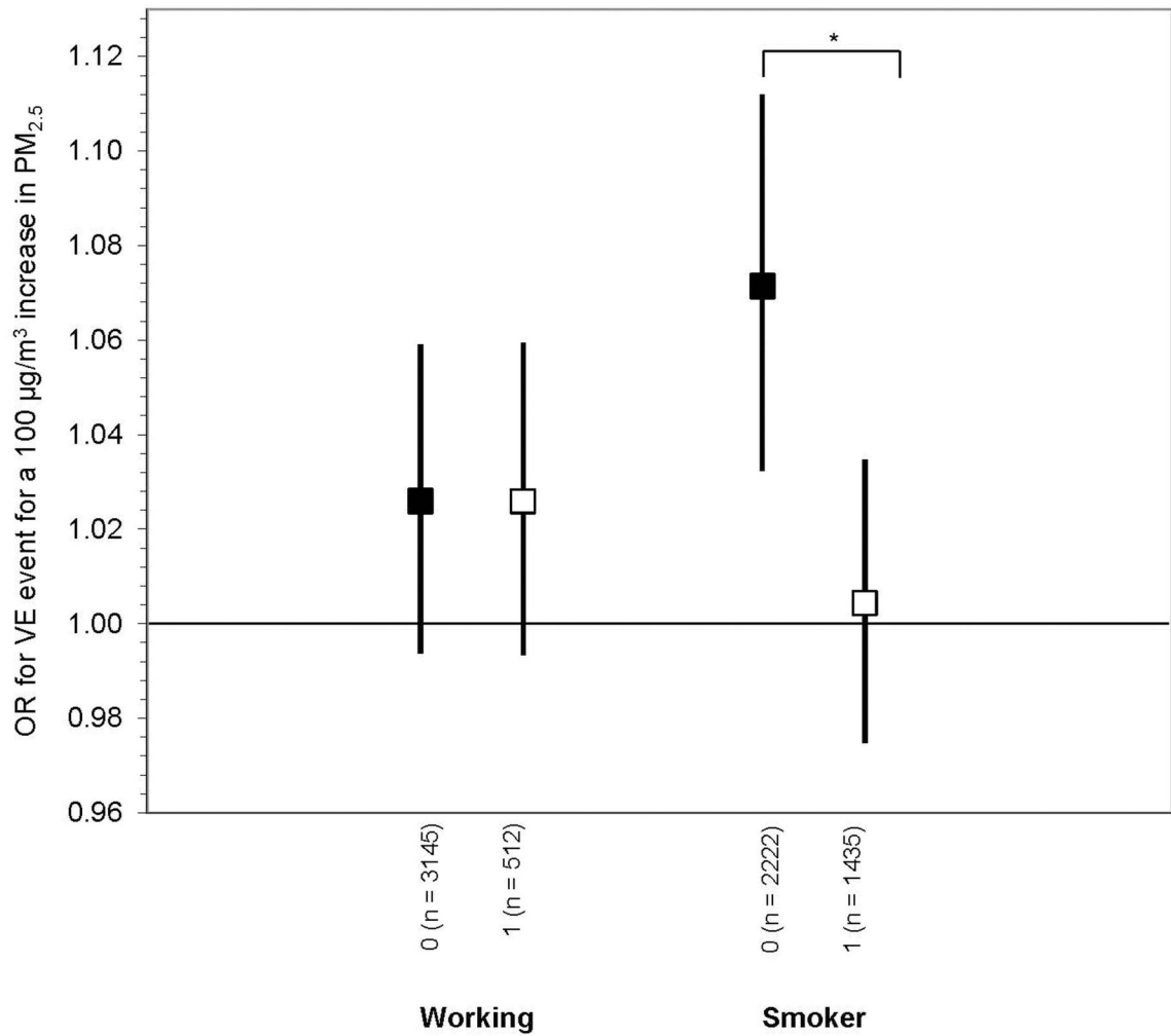
Figure 2. Effect modifiers of the association between ventricular event and PM 2.5 in 6 hours prior. 0 = monitoring hours with characteristic, 1 = monitoring hours without characteristic. All models are adjusted for age, time of day, season and worksite. OR are for a 100 µg/m 3 increase in PM 2.5 in 6 hours prior. Error bars indicate 95% confidence intervals. *Difference in effect is significant at p<0.05
