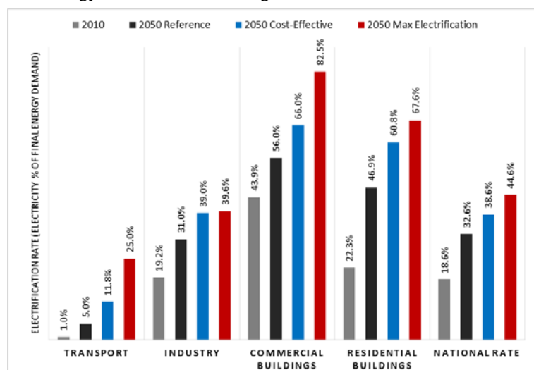
Figure 2. 2010 and 2050 Sectoral Electrification Rates by Scenario
