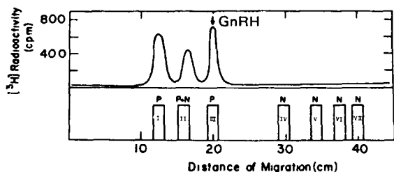
Fig.1. Electropherogram of the degradation products of GnRH. P., Pauli positive; N., ninhydrin positive.
