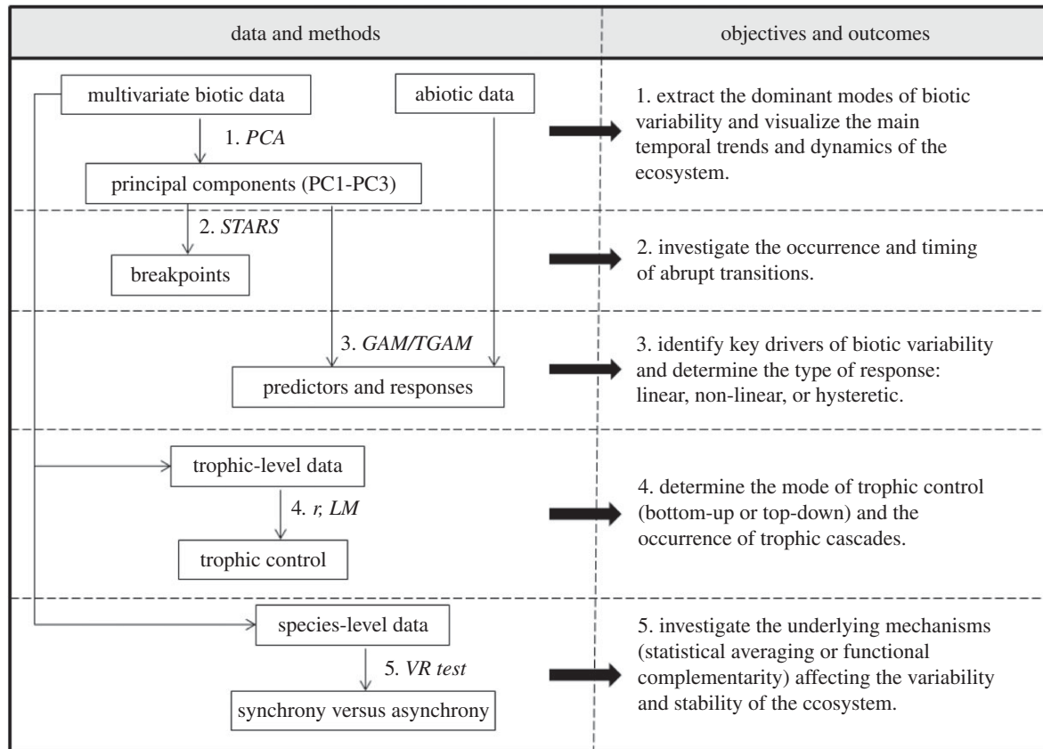
Figure 1. A conceptual figure of the step-wise approach used to characterize abrupt transitions and identify mechanisms promoting resilience and stability in the SCCS. First, PCA was used to extract the dominant trends in a biotic dataset covering multiple trophic levels. Second, a breakpoint analysis (STARS) was applied to investigate potential abrupt transitions in the dominant PCs. Third, nonlinear threshold models (TGAMs) were used to identify key drivers of each PC and determine the type of response, linear, nonlinear or hysteretic [12,13,16]. Fourth, we used correlations and linear regressions to determine the mode of trophic regulation, where positive and negative relationships between adjacent trophic levels indicate bottom-up or top-down control, the latter a sign of trophic cascades. Finally, variance-ratio tests were used to assess the degree of compensation (synchrony/asynchrony) within trophic levels as a means of investigating the underlying mechanisms affecting community variability and stability.
