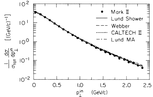
FIG. 22. The p_{\perp}^{\text{in}} distribution of charged particles with respect to the sphericity axis in the event plane in comparison with the models.
