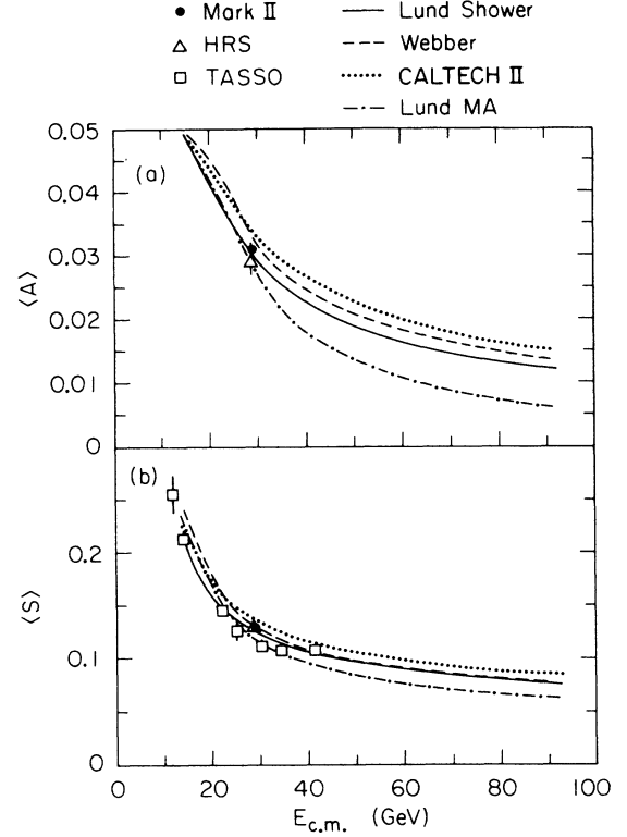
FIG. 27. (a) The \langle A \rangle and (b) \langle S \rangle as a function of E_{c.m.} in comparison with HRS and TASSO results and the model predictions.
