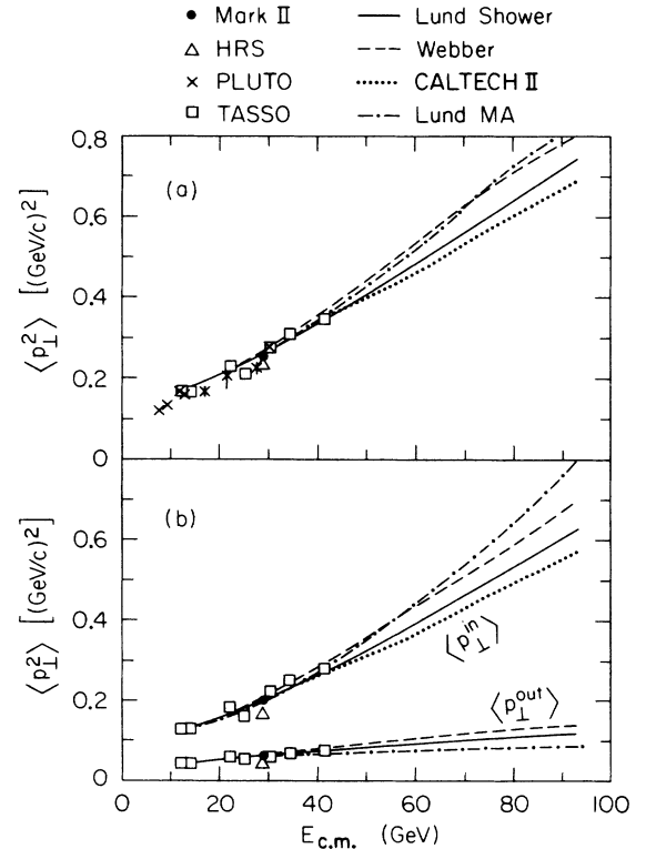
FIG. 32. (a) The \langle p_{\perp}^2 \rangle and (b) the \langle p_{\perp}^{out} \rangle and \langle p_{\perp}^{in} \rangle as a function of E_{c.m.} in comparison with HRS, PLUTO, and TASSO results and the model predictions.
