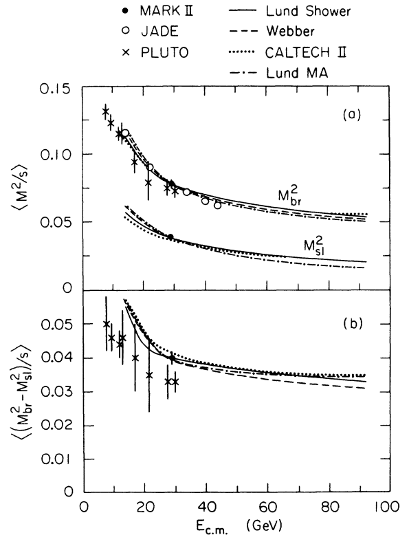
FIG. 28. (a) The \langle M_{br}^2/s \rangle and \langle M_{sl}^2/s \rangle , and (b) \langle (M_{br}^2 - M_{sl}^2)/s \rangle as a function of E_{c.m.} in comparison with PLUTO and JADE results and the model predictions.
