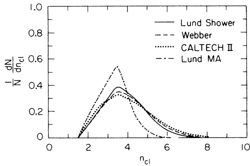
FIG. 40. The predicted number of reconstructed jets or clusters of the models at E_{c.m.} = 93 GeV.
