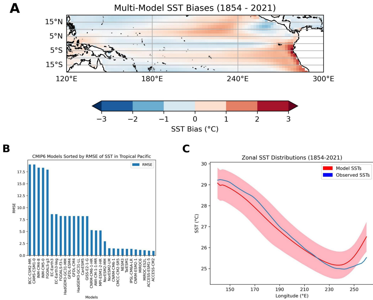
Figure 1. (a) Sea-surface temperature (SST) biases ( ^{\circ}\text{C} ) from the Coupled Model Intercomparison Project, version 6 (CMIP6) multi-model ensemble, averaged December–February (DJF) over 1854–2021. The SST biases were produced by regridding all CMIP6 models to the horizontal grid of the Extended Reconstructed SST Version 5 (ERSSTv5) data set, which was used as the baseline observed SST. Each model is weighted equally to produce the multi-model ensemble average bias (i.e., multiple ensemble members for a given model are averaged before creating the multi-model ensemble average). (b) CMIP6 models ranked according to their root mean square error for tropical Pacific SST, relative to the ERSSTv5 observations. (c) The zonal tropical Pacific SST distribution ( ^{\circ}\text{C} ), averaged over 5^{\circ}\text{N} - 5^{\circ}\text{S} and DJF over 1854–2021. The red line indicates the multi-model mean SST from CMIP6, with the standard deviation of modeled SSTs shaded in pink. Observed SST from ERSSTv5 is shown in blue.
