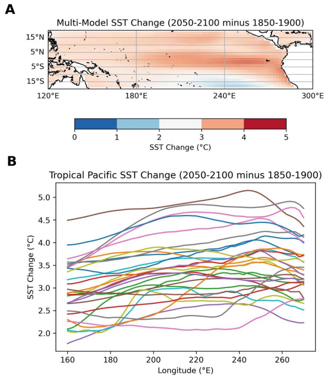
Figure 3. Future change (2050–2100 minus 1850–1900) in sea-surface temperature (SST) ( ^{\circ}\text{C} ) averaged December–February (a) from the Coupled Model Intercomparison Project, version 6 multi-model ensemble and (b) in the tropical Pacific zonal SST distribution ( ^{\circ}\text{C} ), averaged over 5^{\circ}\text{N} – 5^{\circ}\text{S} . (a) As in Figure 1a, each model is weighted equally to produce the multi-model ensemble average SST change. (b) Each line represents the ensemble-mean from one model.
