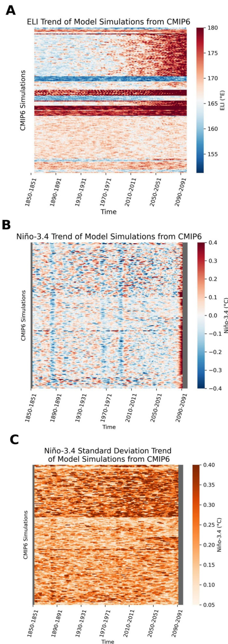
Figure 4. Heatmap displaying trends in the December–February averaged (a) ENSO Longitude Index ( ^{\circ} E), (b) the Niño 3.4 index ( ^{\circ} C), and (c) the standard deviation of the Niño 3.4 index ( ^{\circ} C) over time for all available climate models and ensemble members in the Coupled Model Intercomparison Project, version 6 simulations (i.e., each horizontal stripe represents one ensemble member of a climate model). Lower values in blues indicate (a) La Niña-like conditions, (b) La Niña events, and (c) a decrease in El Niño—Southern Oscillation (ENSO) variability; higher values in reds indicate (a) El Niño-like conditions, (b) El Niño events, and (c) an increase in ENSO variability. (a) The color bar is bounded by 150^{\circ} E and 180^{\circ} E; values less than 150^{\circ} E indicate an extremely strong La Niña event, while values greater than 180^{\circ} E indicate an extremely strong El Niño event. (b), (c) The Niño 3.4 index only runs through 2085, as opposed to 2100, to prevent the appearance of artificial warming trends caused by the rolling climatology at the start and end of the data record. Each of these figures is visually “smoothed” to show the 7-year average value of each index to improve readability.
