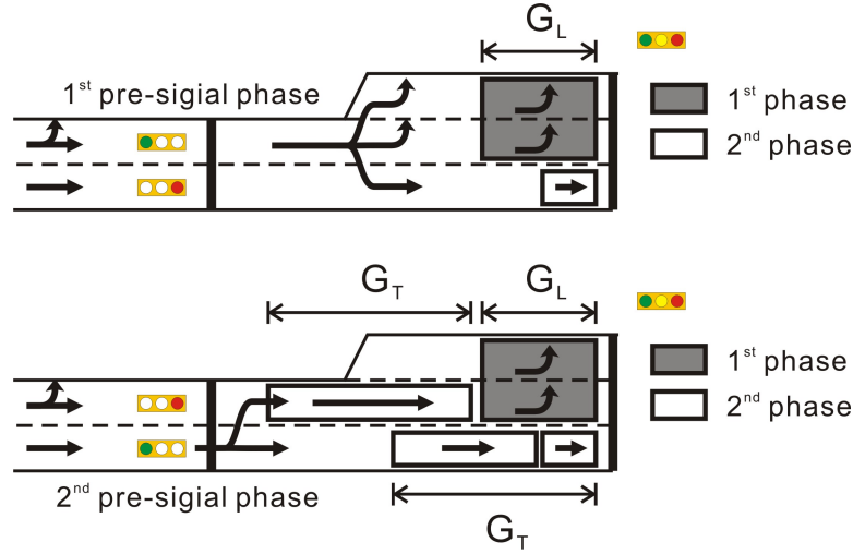
Figure 5.1. Shared lane at the pre-signal. The upper and lower parts of the figure illustrate vehicle movements during the two pre-signal phases respectively.
