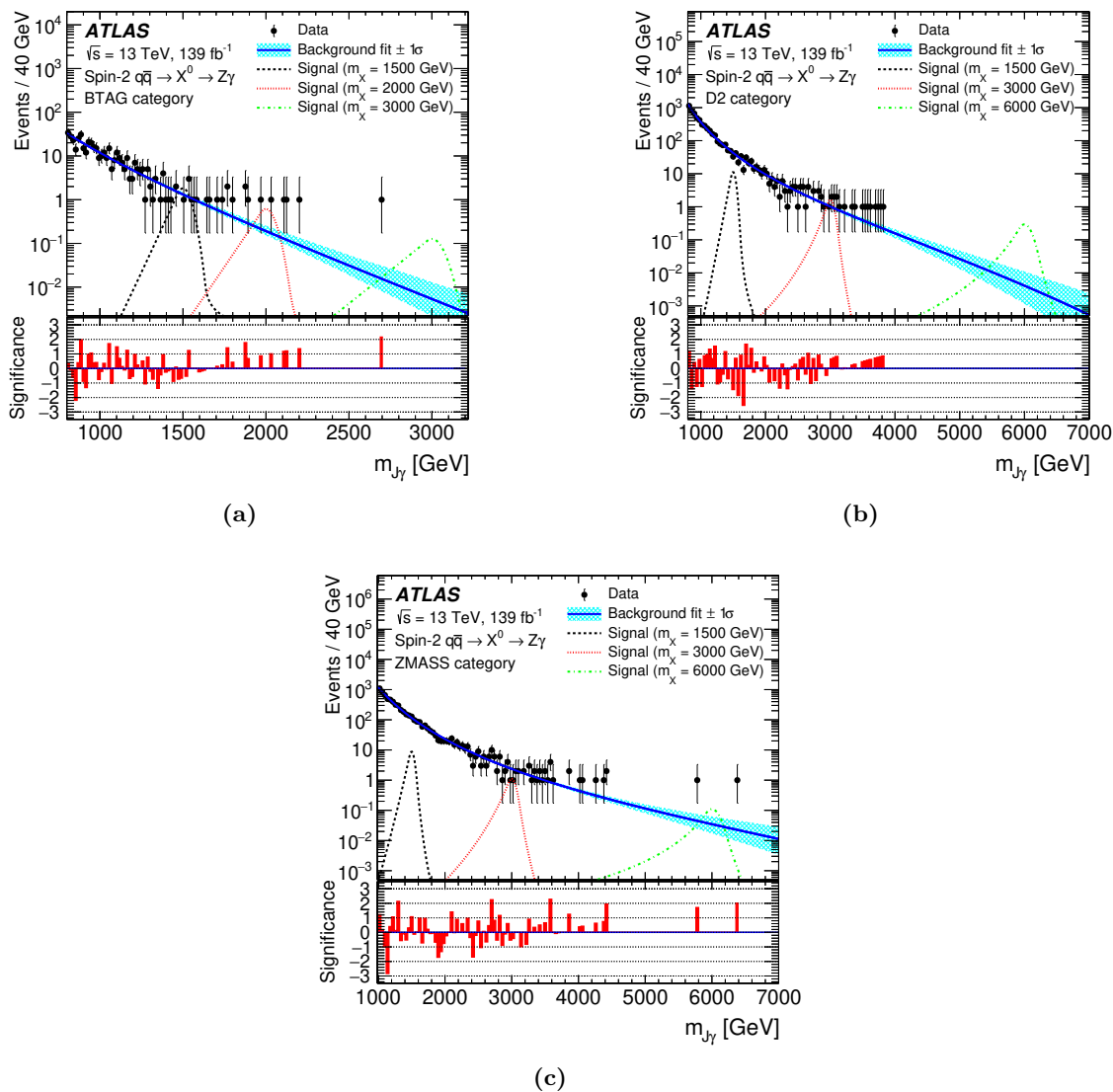
Figure 7. The m_{J\gamma} distributions of data events selected for the spin-2 q\bar{q} \rightarrow X^0 \rightarrow Z\gamma search in the (a) BTAG, (b) D2, and (c) ZMASS categories. The background-only fit function shape is shown as the solid curve overlaid with a shaded band corresponding to statistical uncertainties in background parameters. Various signal shapes with cross-sections corresponding to expected limits obtained in this analysis are shown as dashed lines. The bottom panel presents the binned local significance (filled bars) from a comparison of the data with the background fit using a Poisson model [75].
