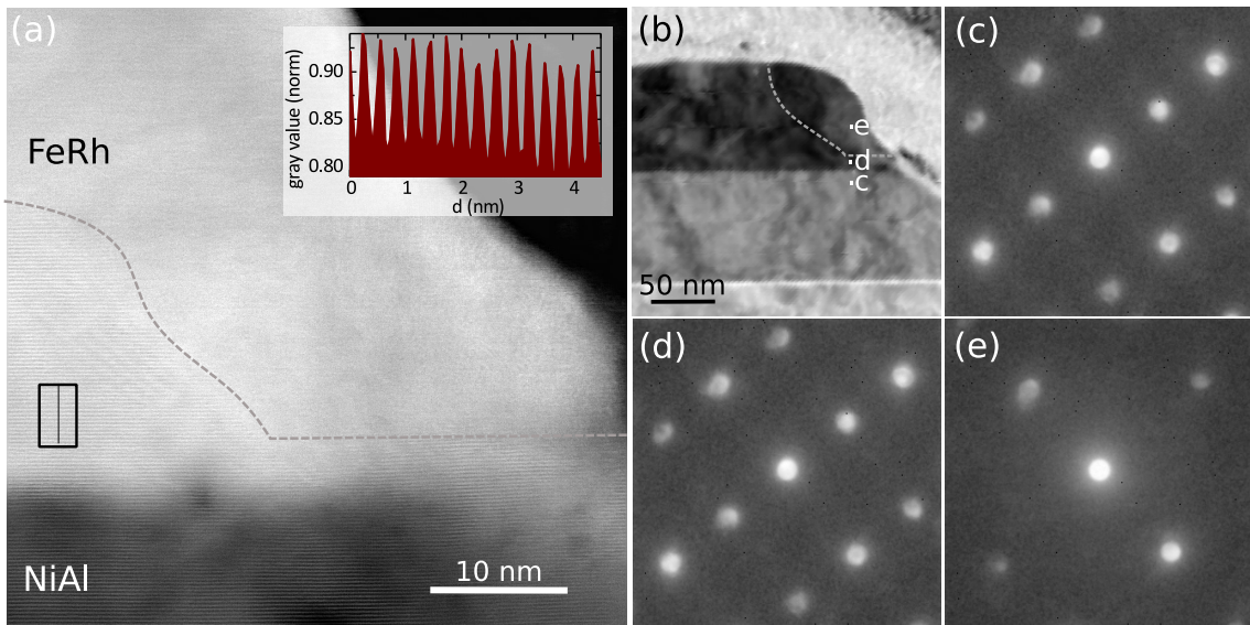
FIG. 8. STEM analysis of the patterned island edge. (a) High resolution STEM image of the right hand edge of the 5 \mu\text{m} island shown in Fig. 1(d). The inset is a vertical line scan over the indicated region showing lattice fringes. These fringes are not observed in the edge grain region above and right of the dashed grey line. (b) Bright field image with diffraction contrast over a larger region and grey dashed line showing continuation of grain. Nanodiffraction images of points indicated in (b) are shown in (c)-(e).
