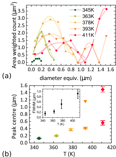
FIG. 5. Characteristic sizes of FM domains. (a) Area weighted histogram of the domain size at various temperatures during the heating process. See text for details. (b) Peak centres of Gaussian peak fits to the histograms in (a), inset the peak full width half maxima (FWHM) are plotted.
