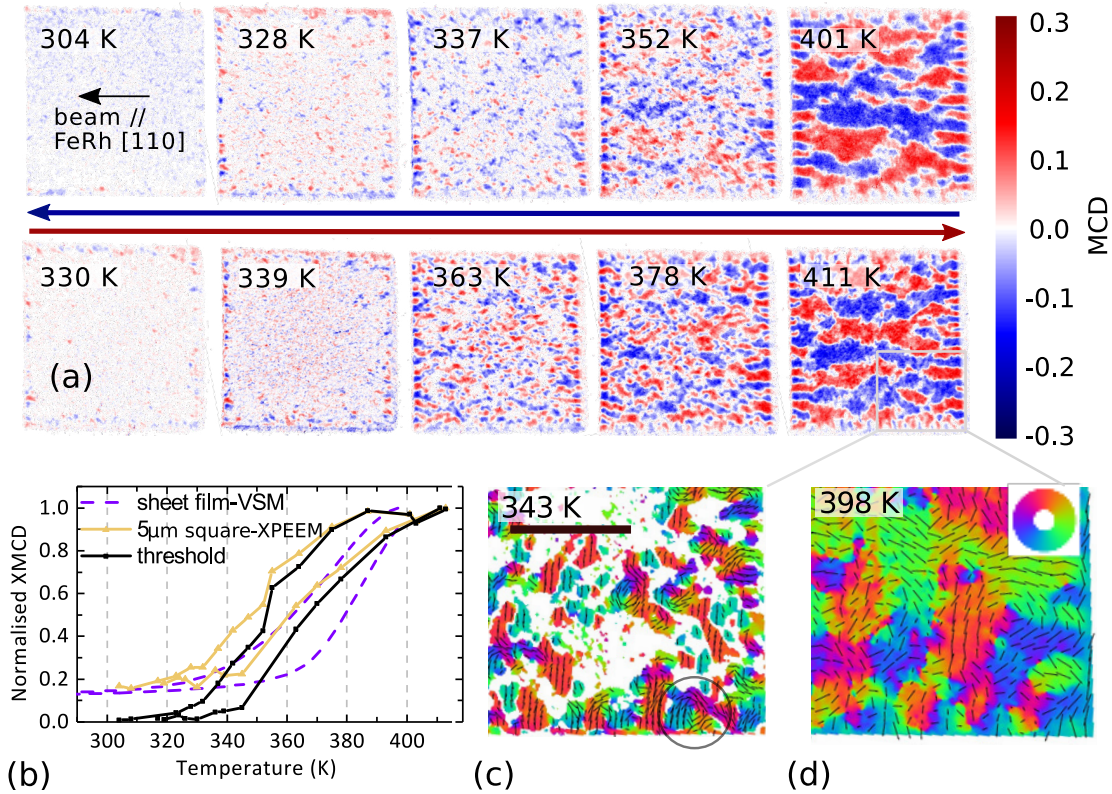
FIG. 3. XPEEM imaging of FM domains. (a) Magnetic dichroism images of an island of side 5 \mu\text{m} shown as a function of temperature during the cooling process (upper row of images) and the heating process (lower row). The beam direction and magnetic sensitivity are shown in the top left image. (b) The integrated absolute XMCD signal as a function of temperature and in comparison to a VSM measurement. Both signals are normalised to the saturation value. The thresholded signal is also shown, see text for details. (c) and (d) Vector magnetisation maps of the bottom right portion of the 5 \mu\text{m} island during heating. The inset scale bar on (c) is 1 \mu\text{m} . The colour represents the vector direction indicated in the colour wheel and the length of the arrows represent local XMCD magnitude. A vortex state is highlighted in (c).
