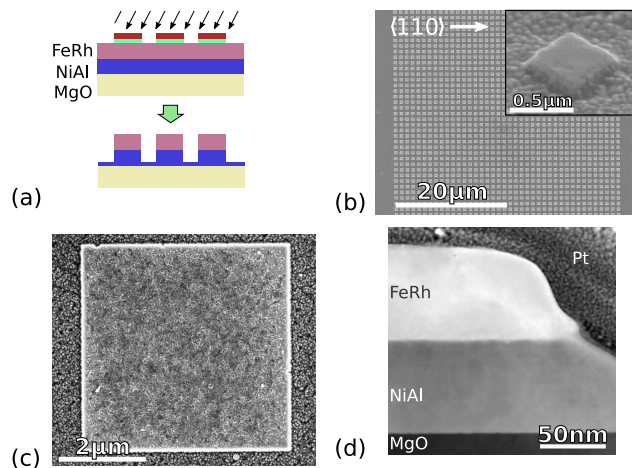
FIG. 1. FeRh nanopatterned islands. (a) Diagram of the nanofabrication process, see the text for full explanation. (b) SEM image of the array of 0.5 \mu\text{m} squares. Inset is a close up image of one of the islands taken at a 45 degree angle to the film plane. The damage to the NiAl layer from the ion milling is seen. (c) In-lens detection SEM image of a 5 \mu\text{m} island highlighting grain edges. (d) Cross-section TEM on the edge of a 5 \mu\text{m} island using annular dark field contrast.
