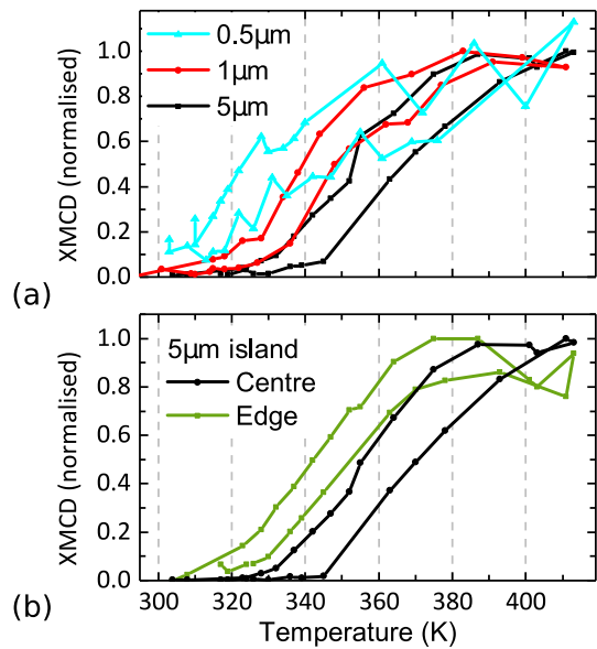
FIG. 6. Phase transition measured by XMCD. (a) Absolute dichroism integrated over the entire island for 0.5, 1 and 5 \mu\text{m} island sizes shown on the same scale. For the smaller two sizes an average signal over four FeRh islands have been plotted. (b) The integrated dichroism signal vs. temperature for the 5 \mu\text{m} island. The integral is over the edge and central area of the island as indicated.
