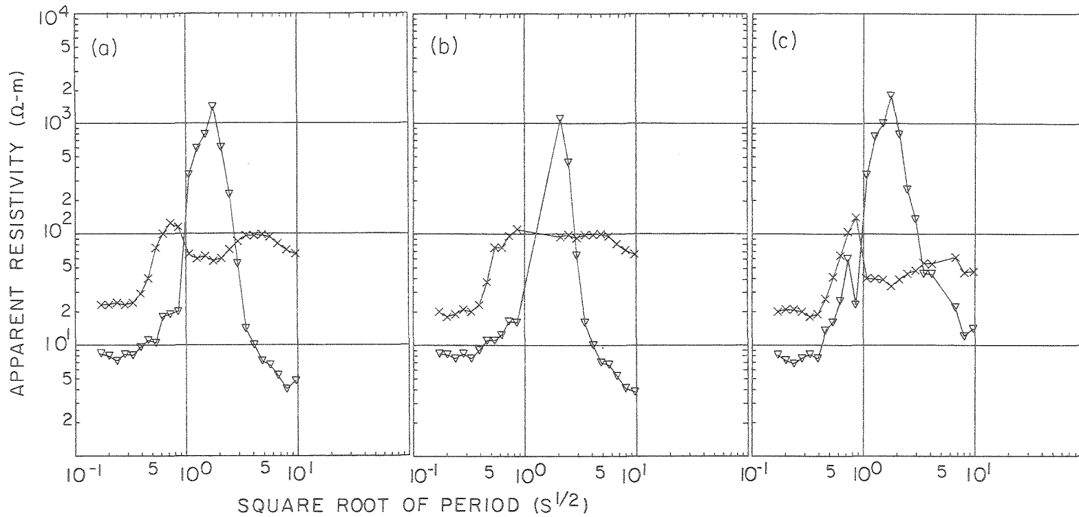
Fig. 8. Rotated apparent resistivities versus square root of period from the one reference channel analysis, method III, of the 1976 data from location 2. a) substitution of \overline{E_i^1 E_i^*} for the electric field autopowers in \underline{Z}^E , b) equations (4.40) with \underline{G} = \underline{Z} , c) equations (4.40) with \underline{G} = \underline{Y} and \underline{Z} = \underline{G}^{-1} .
