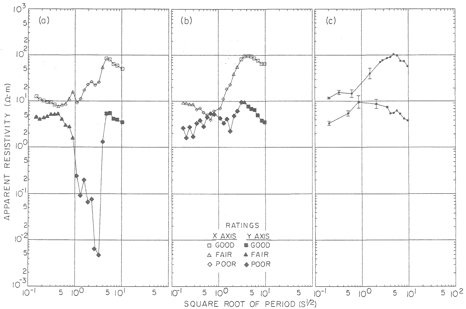
Fig. 3. Rotated apparent resistivities versus square root of period for location 2. a) 1975 data using Z^H , b) 1976 data using Z^H , c) 1976 data with double average analysis, method IV.
