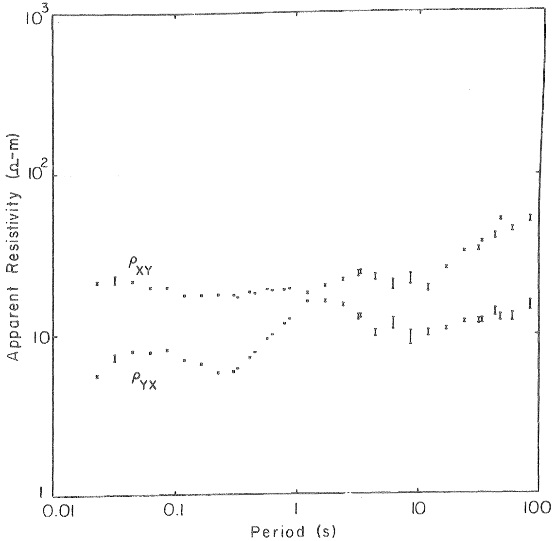
Fig. 27. Rotated apparent resistivities from Z^R and their probable errors versus period, Lower La Gloria.
