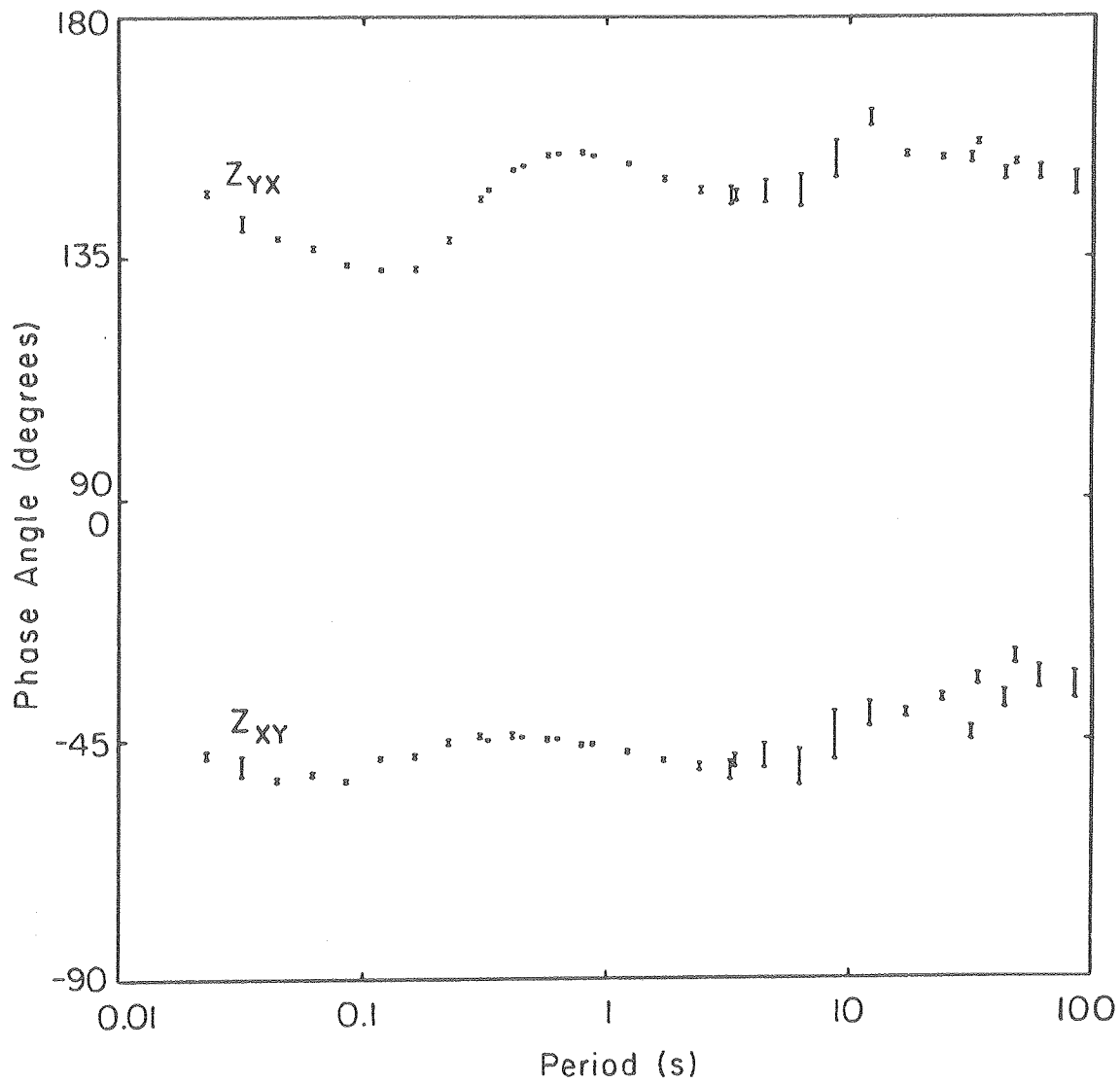
Fig. 29. Phases from \underline{Z}^R and their probable errors versus period, Lower La Gloria.
