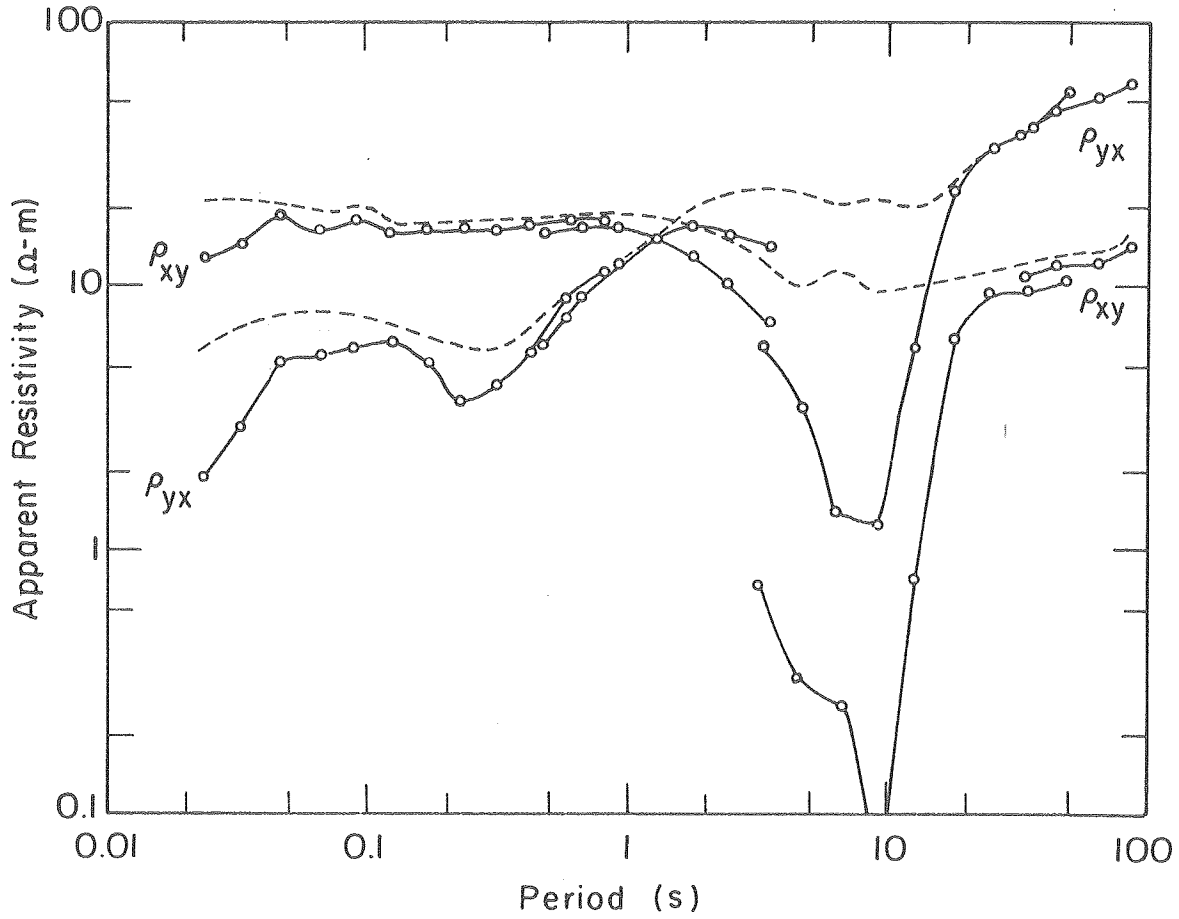
Fig. 25. Rotated apparent resistivities from \underline{Z}^H versus period. Lower La Gloria. ----- remote reference results.
