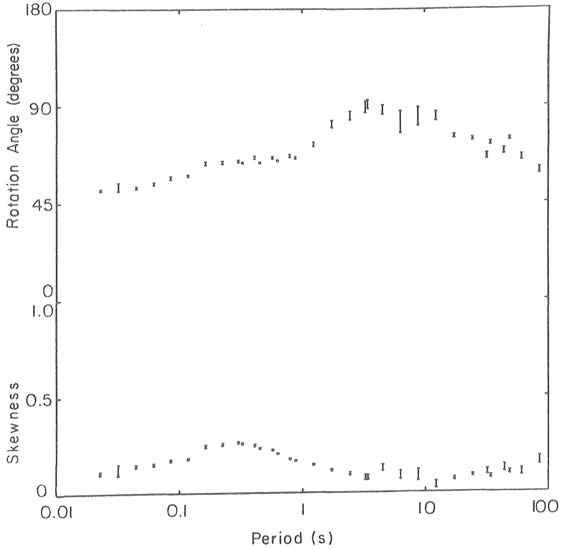
Fig. 28. The angle between magnetic north and the \hat{x} axis of the coordinate system aligned with the apparent strike direction and the skewness from Z^R with their probable errors versus period, Lower La Gloria.
