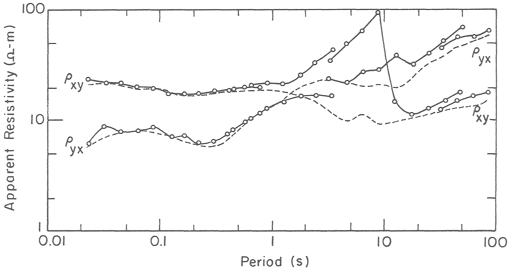
Fig. 23. Rotated apparent resistivities from Z^E versus period, Lower La Gloria. ----- remote reference results.
