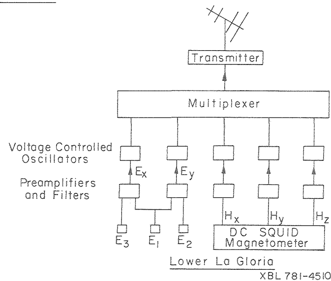
Fig. 10. Block diagram of data acquisition.
