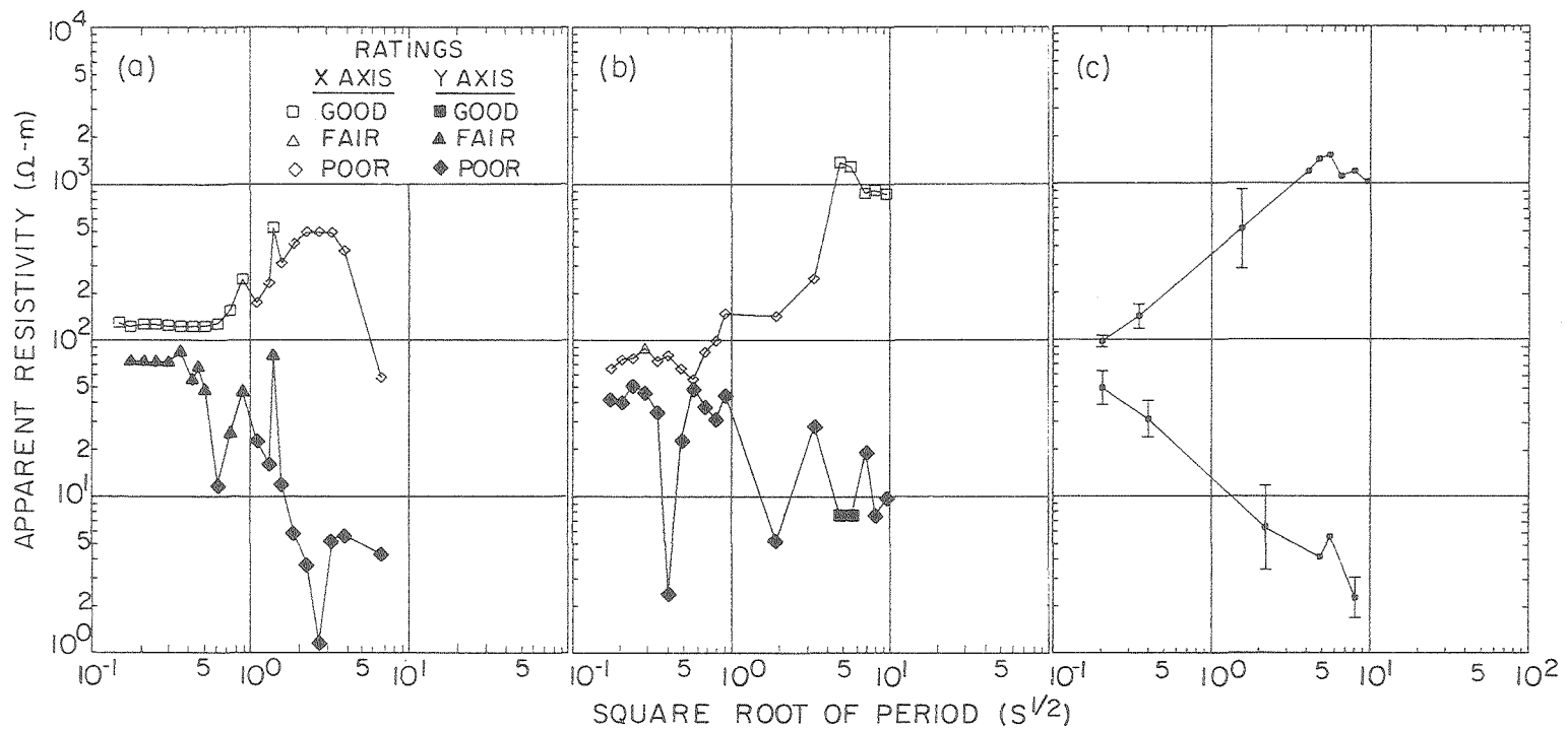
Fig. 4. Rotated apparent resistivities versus square root of period for location 3. a) 1975 data using Z^H , b) 1976 data using Z^H , c) 1976 data with double average analysis, method IV.
