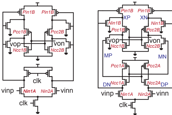
(a) Double-tail sense amp (DTSA) [5]
