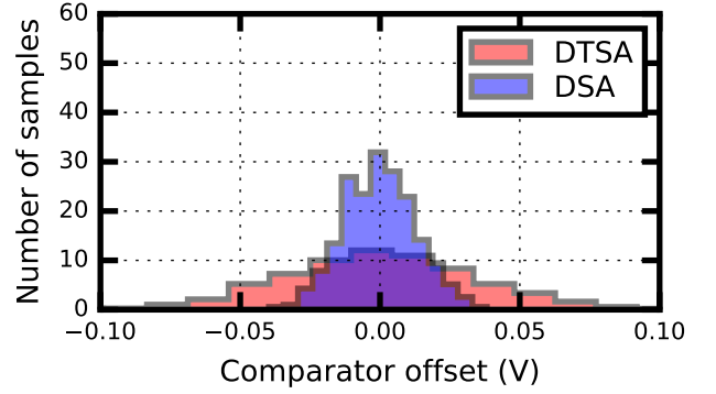
Fig. 8. Measured offset of DTSA and DSA for V_{DD} = 1V (top) and V_{DD} = 0.7V (bottom).
