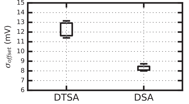
Fig. 11. Spread of the measured standard deviation of the offset across all dies for each comparator type.
