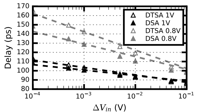
Fig. 5. Simulated delay across input voltage difference and least-square best-fit lines (dashed) for equal fanout DTSA and DSA.
