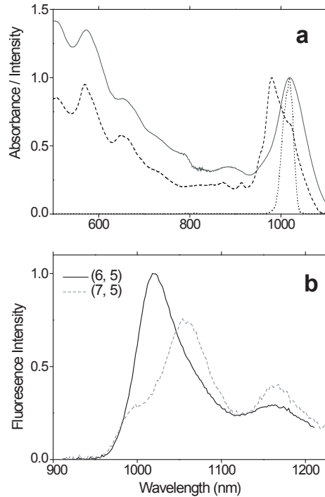
Figure 8.1. a) Linear absorption spectra of the SWNT/PVP composite film (solid line) and the D 2 O solution of the NaDDBS dispersed SWNTs (dashed line), which was used to fabricate the SWNT/PVP film. The dotted line is the laser pulse spectrum. Both absorption spectra are normalized at the peaks of the E_{11} transitions, and the laser pulse spectrum is scaled to match the E_{11} peaks. (b) Steady-state fluorescence emission spectra measured for the SWNT/PVP film upon resonant excitation of the E_{22} transitions of the (6, 5) and (7, 5) tubes at 572 and 655 nm, respectively.
