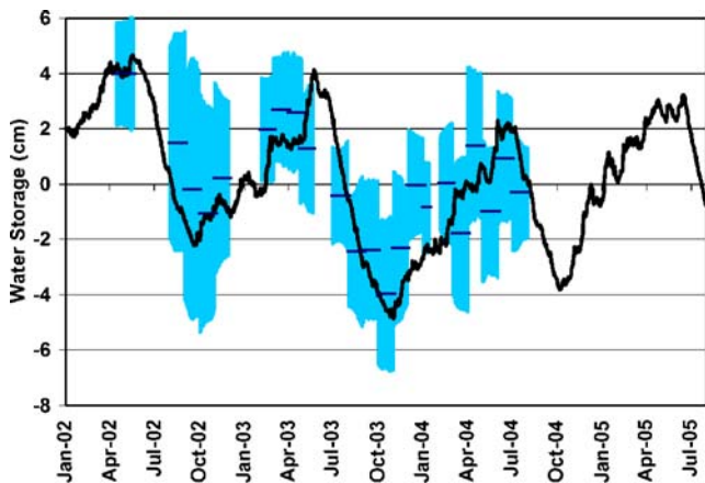
Fig. 3 Groundwater storage estimated from GRACE and land surface models using Eq. 1 ( dark blue bars ), and based on monitoring well observations ( black line ), as deviations from their GRACE-period means, presented as equivalent layers of water (cm) averaged over the Mississippi River basin. The length of the dark blue bars represents the extent of the GRACE averaging period. The light blue shaded area depicts the uncertainty in the GRACE-GLDAS estimates
