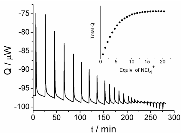
Figure 3. ITC data for the addition of a 90 mM solution of \text{NEt}_4^+ into a 1 mM solution of 1 . Inset: total heat vs. equiv. \text{NEt}_4^+ .
