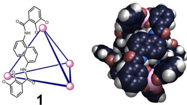
Figure 1. Schematic of the [\text{Ga}_4\text{L}_6]^{12-} framework, only one ligand is shown for clarity (left). Space-filling model of 1 as viewed down the 2-fold axis (right).
