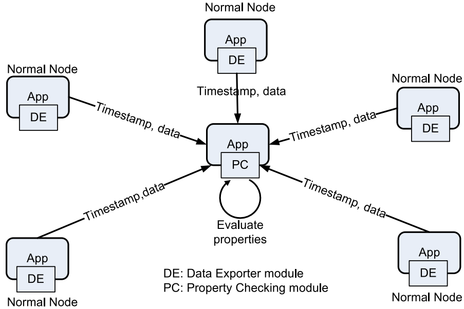
Figure 3.3: Centralized approach for evaluating properties
