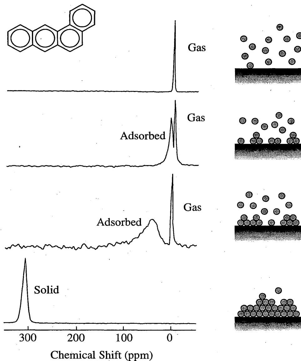
Figure 6.1: ^{129}\text{Xe} NMR spectra of laser-polarized xenon adsorbed onto powdered benzenanthracene [46]. (a) Spectrum showing only gaseous xenon (298 K, 20 torr). (b,c) Spectra showing both gaseous and adsorbed xenon (158 K, 21 torr for (b), 153 K, 22 torr for (c)). (d) Spectrum showing only solid xenon (123 K). Figure courtesy of Thomas Meersmann.
