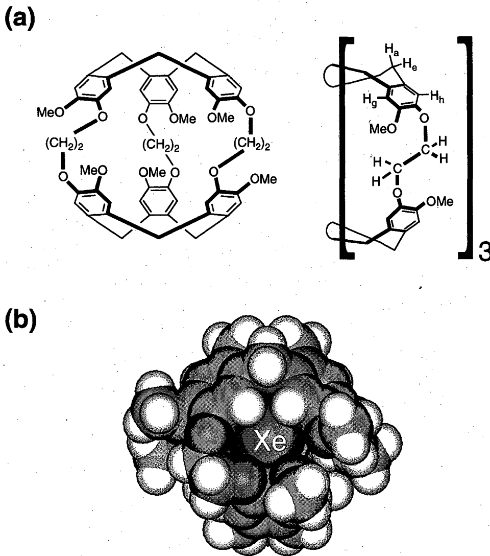
Figure 5.5: (a) (Color) Structure of cryptophane-A and atom labeling used in the 1 H NMR spectrum of Fig. 5.9(a). The assignment of the 1 H signals of the spacer bridges is discussed later in the chapter. (b) CPK model of one possible conformation of cryptophane-A with a xenon atom placed within the binding cavity.
