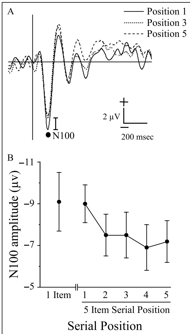
Figure 4. N100 component as a function of serial position. (A) Potentials to in-set probes that were presented in the 1st, 3rd, and 5th serial positions of the memory set (bandpass filtered 1–16 Hz). (B) Plot of N100 amplitudes for in-set probes in the 1-item memory set and across serial positions in the 5-item memory set. N100 amplitudes were equivalent for the 1-item set and the 1st serial position of the 5-item set, and had significantly smaller amplitudes for serial Positions 2 through 5. Error bars indicate standard error.
