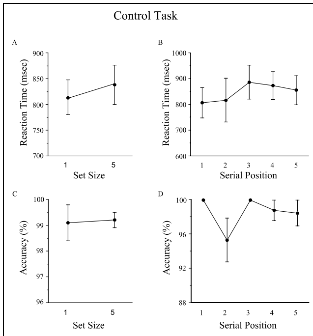
Figure 8. Behavioral results from Experiment 2 (control task). Reaction time as a function of set size (A) and serial position (B). Unlike Experiment 1, reaction time was not significantly different as a function of set size or serial position. Accuracy as a function of set size (C) and serial position (D). Error bars indicate standard error.
