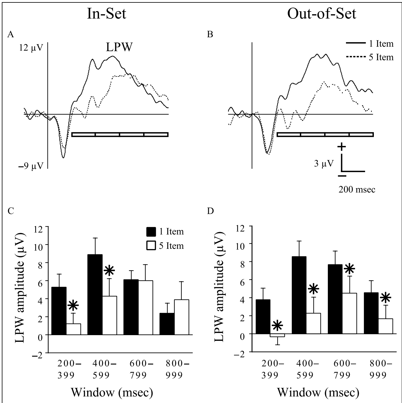
Figure 7. Grand average potentials (DC—16 Hz) to probes in 1- and 5-item memory sets. Potentials for in-set (A) and out-of-set (B) probes (DC—16 Hz) show amplitude differences between 1- and 5-item memory sets, with larger LPW amplitudes in the 1-item memory set. LPW amplitudes for 1- and 5-item memory sets are shown for in-set (C) and out-of-set (D) probes. Error bars show standard error.
