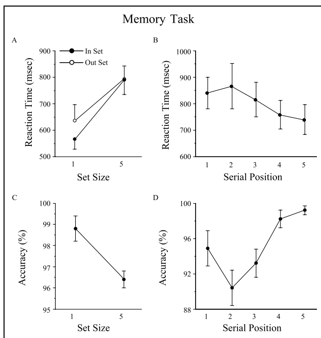
Figure 2. Behavioral results from Experiment 1. Reaction time as a function of memory set size (A) and serial position (B) in the 5-item memory set. Reaction time was significantly longer for the 5- versus 1-item memory set. Reaction time was also significantly different as a function of serial position, which indicates a recency effect. Accuracy as a function of memory load (C) and serial position (D). Accuracy was significantly reduced for the 5- versus 1-item memory set and showed a significant recency effect across serial positions. Error bars indicate standard error.
