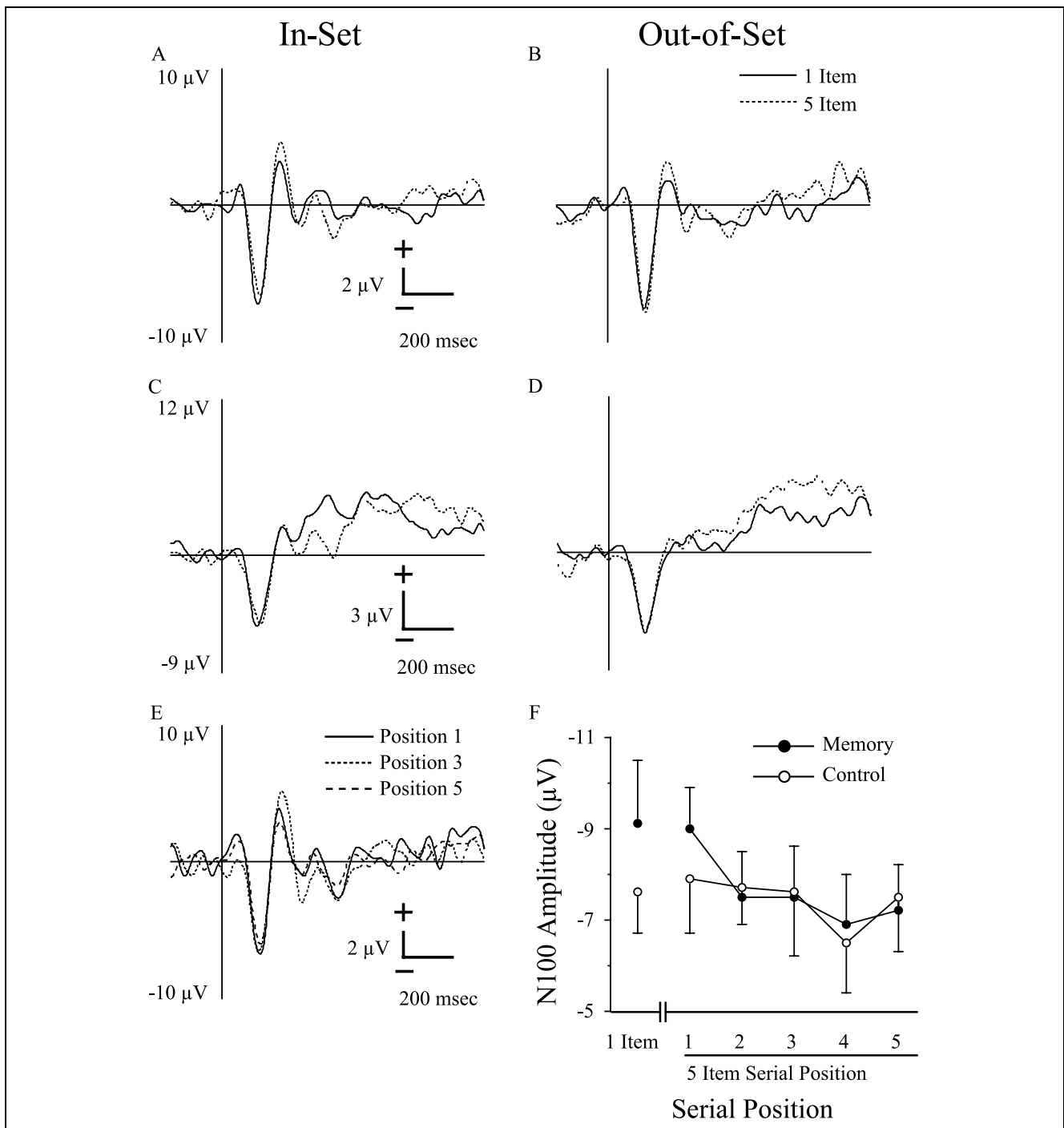
Figure 9. Potentials to probes in Experiment 2 (control task). Bandpass filtered potentials (1–16 Hz) to in-set (A) and out-of-set (B) probes. In-set and out-of-set status of probes was not relevant to the even/odd number classification task, but in-set and out-of-set averages were compiled for comparison with Experiment 1. Low-pass filtered potentials (DC–16 Hz) for in-set (C) and out-of-set (D) probes, illustrating the absence of a notable LPW (compare with Figure 7A and B). N100 tracings (E) and amplitude plots (F) as a function of serial position in Experiment 2. There were no significant effects of serial position on N100 amplitude or latency. Panel F shows N100 amplitudes in Experiment 1 (memory task) and Experiment 2 (control task). Note that N100 amplitudes were larger in the memory task versus control task in the 1-item set size and the 1st serial position of the 5-item set. Error bars indicate standard error.
