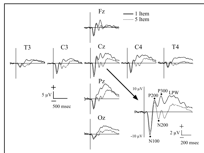
Figure 3. Event-related potentials to probes at all electrode sites for 1- and 5-item memory sets. Inset from Cz site shows measured components. Potentials were low-pass filtered (DC–16 Hz).
