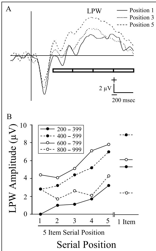
Figure 5. LPW component as a function of serial position. (A) Potentials to in-set probes that were presented in the 1st, 3rd, and 5th serial positions of the memory set. (B) Plots of LPW amplitudes from four 200-msec windows (starting 200 msec after probe presentation) as a function of serial position. LPW amplitudes for probes in the 1-item memory set are also presented for comparison.
