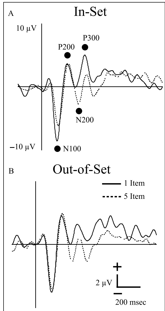
Figure 6. Grand average potentials (1–16 Hz) in the 1- and 5-item memory sets for in-set (A) and out-of-set (B) probes. The N100, N200, and P300 components had significantly smaller amplitudes and longer latencies for the 5-item memory set relative to the 1-item memory set.
