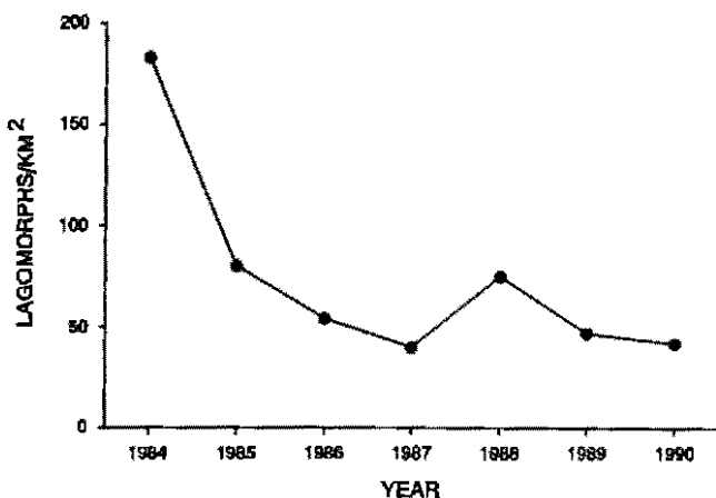
Figure 2. Summer lagomorph density estimates from 1984 to 1990, Naval Petroleum Reserve #1, California.
