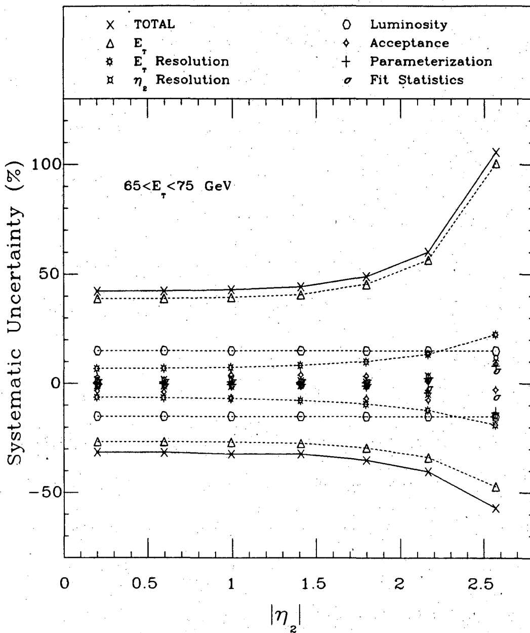
Figure 6.5: The systematic uncertainties on the two jet differential cross section are shown for a single E_t interval. For each |\eta_2| value the independent sources of systematic uncertainty are shown and the total systematic uncertainty, from adding the individual uncertainties in quadrature, is also shown. Important systematic uncertainties are joined by dotted lines, and the total systematic uncertainty is joined by a solid line, to illustrate the way the uncertainty grows with |\eta_2| .
