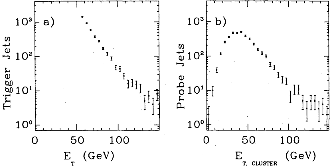
Figure 4.10: The E_t distributions of the two leading jets from the Medium Threshold sample. a) The “true” jet E_t of the trigger jet. b) The uncorrected cluster transverse energy of the probe jet. The distributions contain no corrections for E_t resolution smearing.
