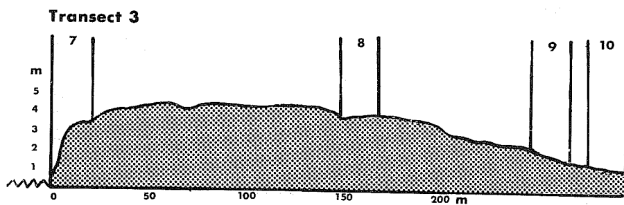
FIG. 3 - Profiles of the levee at Shoonto North study site from the river to the dhesteege edge, showing the position of vegetation plots.
