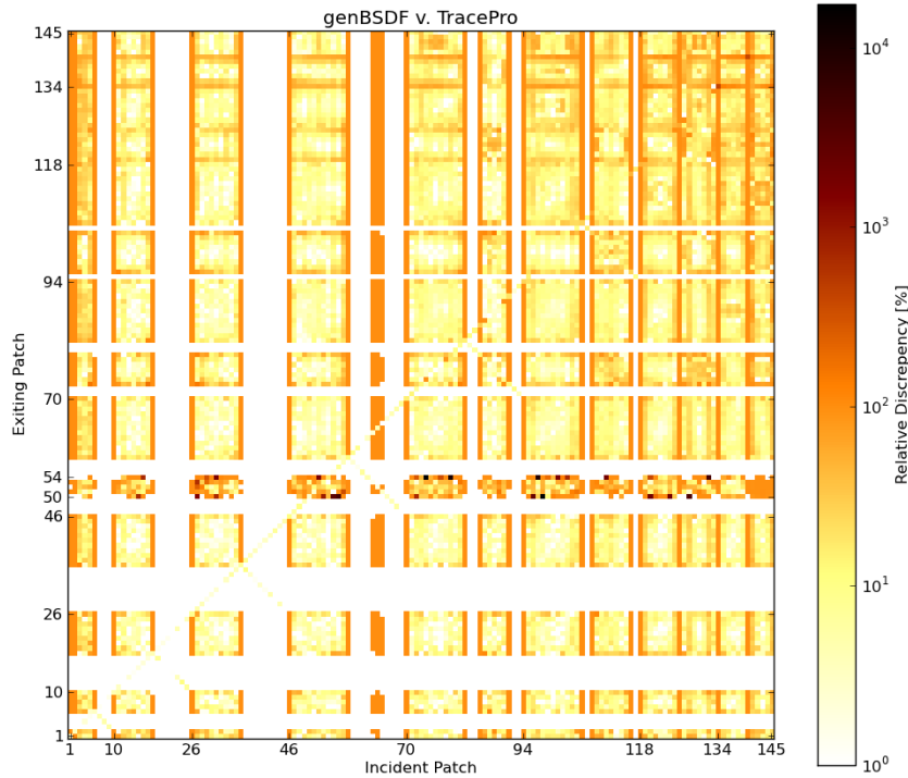
Fig. 5. Percent difference between genBSDF- and TracePro-generated BSDFs (transmission) for flat specular blinds positioned at a horizontal angle.
