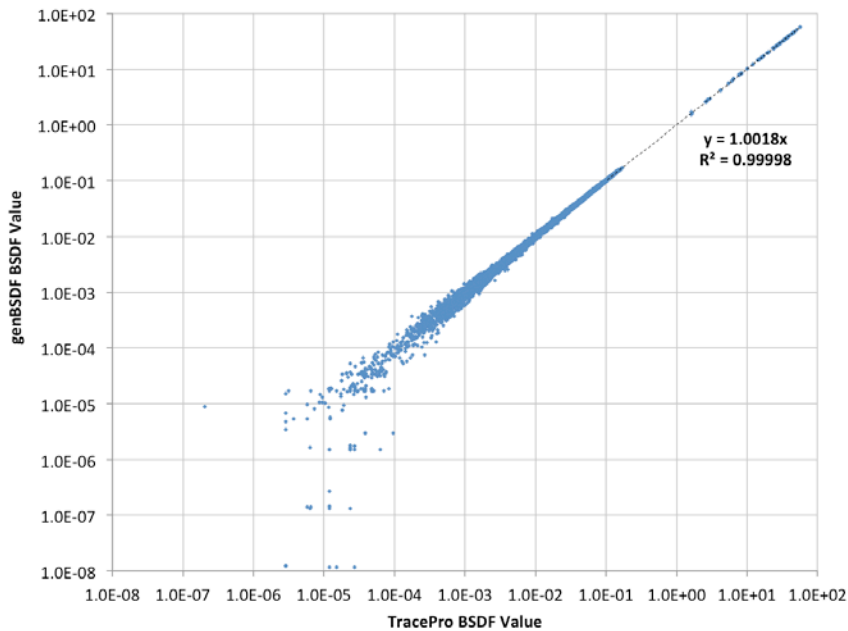
Fig. 6. Scatter plot of modified genBSDF (with a collimated source) versus TracePro BSDF values for flat specular blinds. The 21,250 transmission values are correlated with a linear regression fit ( r^2=0.99998 ).
