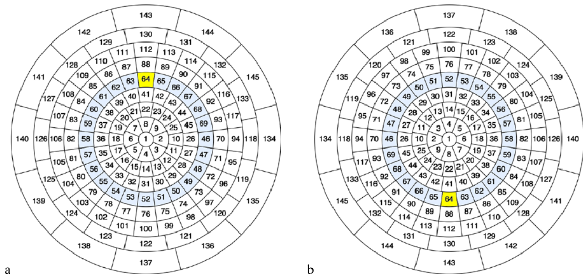
Fig. 1. Angular projection of Klems angle basis viewed from the incident side for (a) incident (normal direction out of the page) and (b) transmitted hemispheres (normal direction into the page). The blue shaded regions indicate a Klems “theta band” which is all the patches with the same theta angles. A “phi division” is a single patch in the theta band (eg shaded in yellow). Note that the numbering scheme of the patches is different for the two hemispheres. This numbering is chosen to allow a specular beam to be described by the same patch number for incident, reflected and transmitted directions.
