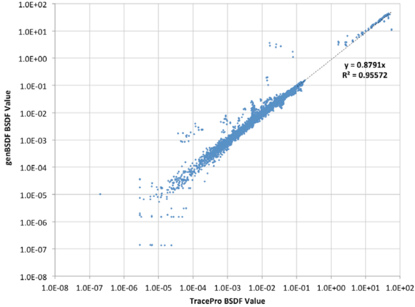
Fig. 4. Scatter plot of the genBSDF results versus the analytically derived, TracePro BSDF values for the specular Venetian blind. The 21,250 transmission values are correlated with a linear regression fit ( r^2=0.95572 ).
