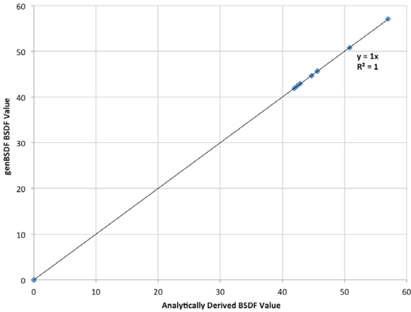
Fig. 3. Scatter plot of the genBSDF results versus the analytically derived BSDF values for air. The 21,250 transmission values are correlated with a linear regression fit ( r^2=1.0 ).
