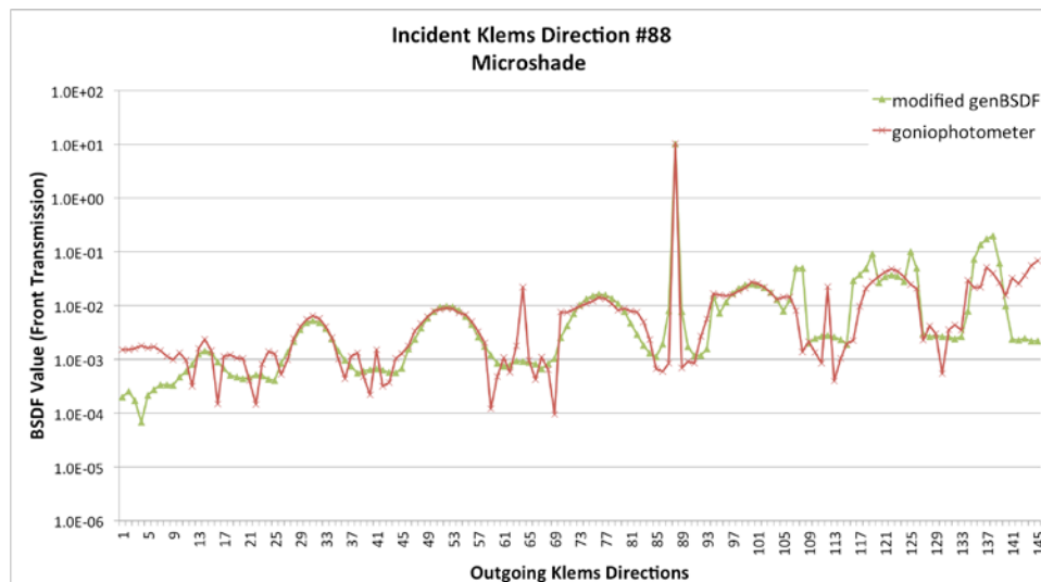
Fig. 9. Chart of measured and simulated BSDF values of micro-perforated shade for Klems incident patch number 88.
