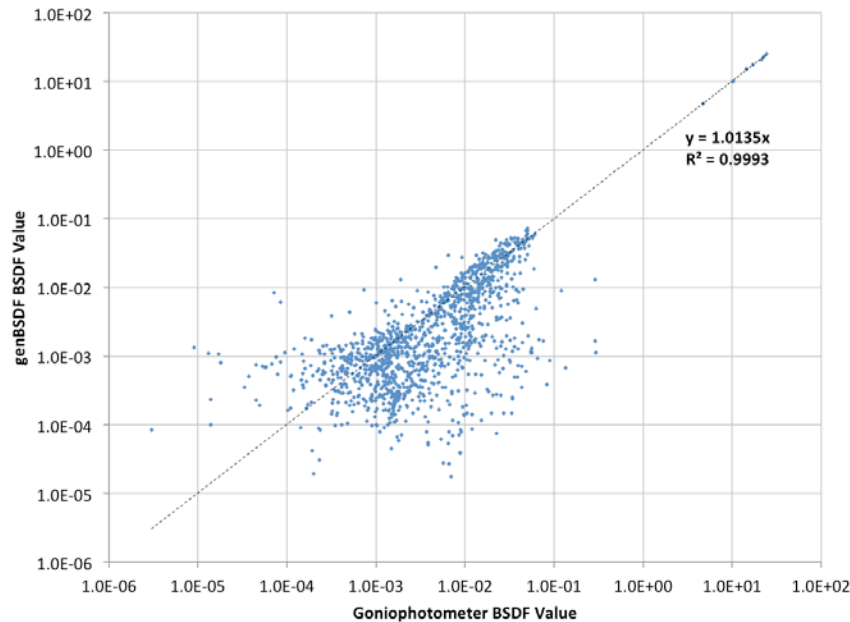
Fig. 11. Scatter plot of BSDF values from modified genBSDF (with collimated source) versus goniophotometer measurements for the micro-perforated shade. The 21,250 transmission values are correlated with a linear regression fit ( r^2=0.9993 ).
