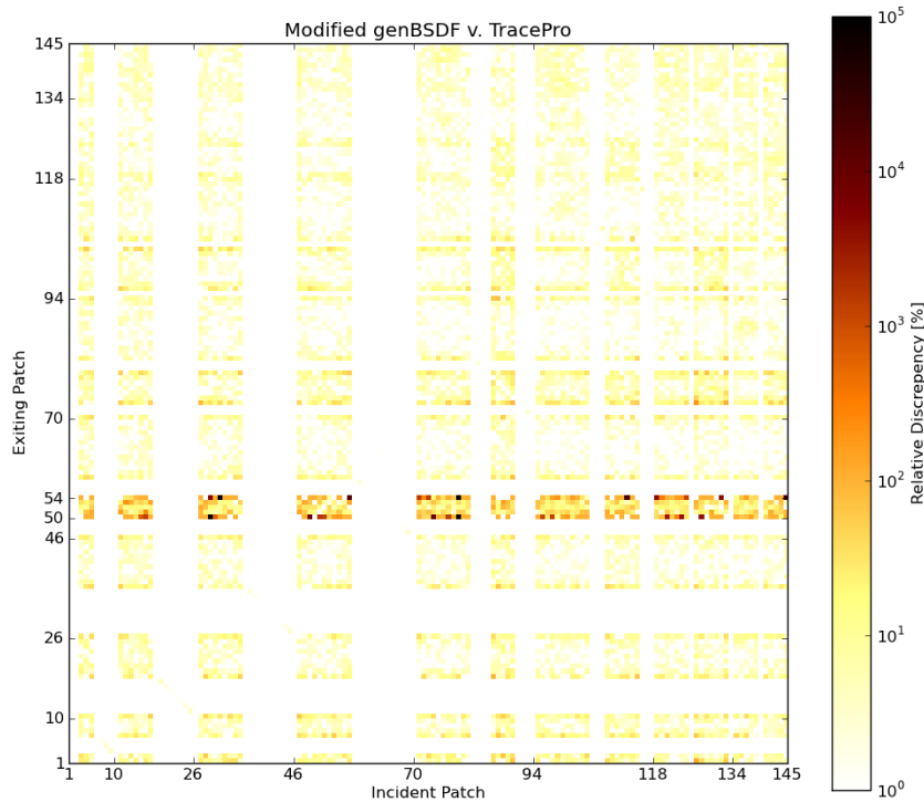
Fig. 7. Percent difference between modified genBSDF- and TracePro-generated BSDFs (transmission) for flat specular blinds positioned at a horizontal angle.
