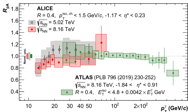
Fig. 6 Nuclear modification factor ( R_{pA} ) of isolated prompt photon production in p-Pb collisions at \sqrt{s_{NN}} = 5.02 and 8.16 TeV shown together with a measurement by the ATLAS collaboration in p-Pb collisions at \sqrt{s_{NN}} = 8.16 TeV [52]. For illustration purposes, the data points at \sqrt{s_{NN}} = 5.02 TeV are displaced by \Delta p_T = +300 MeV/c. The normalisation uncertainties are denoted as coloured boxes around unity
