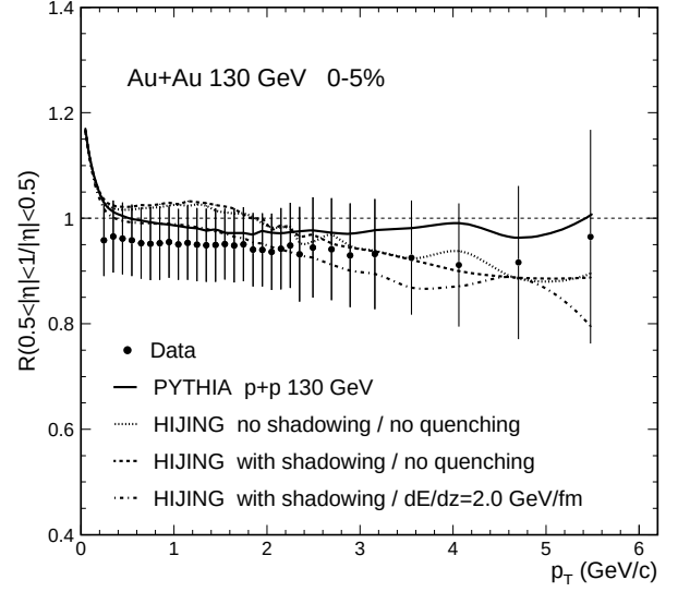
FIG. 6: Ratio of p_T distribution within 0.5 < |\eta| < 1 to that within |\eta| < 0.5 in the 0–5% most central bin. Points are measurements and error bars include statistical and remaining systematic uncertainties. Curves are described in the text.
