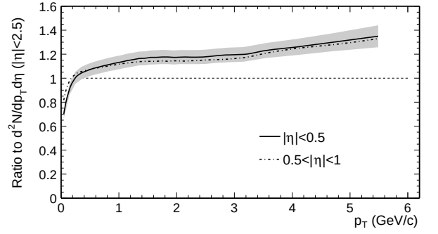
FIG. 2: \eta acceptance correction function from model calculations: ratios of p_T spectra in two different \eta regions to that within |\eta| < 2.5 , in which the UA1 Collaboration published its inclusive charged particle p_T spectra.
