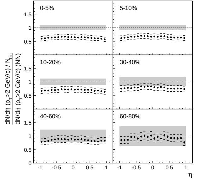
FIG. 7: dN/d\eta distributions for p_T > 2 GeV/c and -1 < \eta < 1 scaled by N_{bin} and divided by the NN reference.
