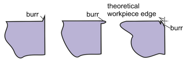
Fig. 4. Examples of burr definition according to [47].
