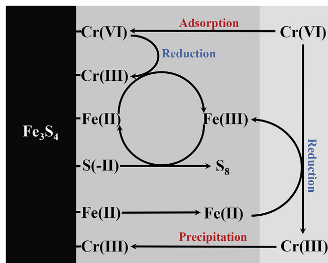
Scheme 1. Proposed Cr(VI) removal mechanism with magnetic \text{Fe}_3\text{S}_4 .
