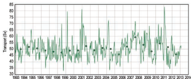
Fig. 3.19. Altimetry-derived transport of the Agulhas Current from a combination of sea height anomaly and climatological hydrography. (Source: http://www.aoml.noaa.gov/phod/altimetry/cvar/agu/index.php )
