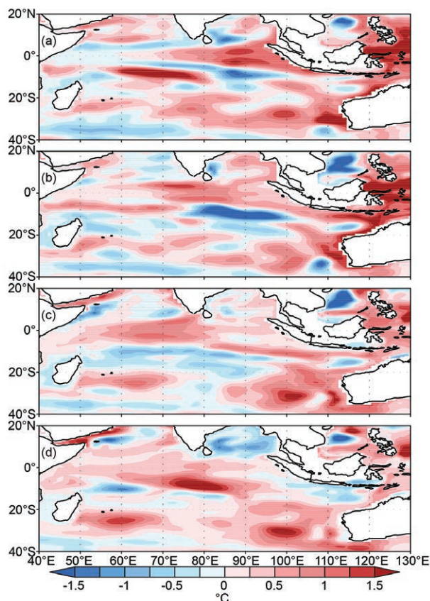
FIG. 4.39. Upper 300 m mean ocean temperature anomalies ( ^{\circ}\text{C} ) based on the NCEP ocean reanalysis during (a) DJF 2011/12, (b) MAM 2012, (c) JJA 2012, and (d) SON 2012. (Source: www.cpc.ncep.noaa.gov/products/GODAS/ .)
