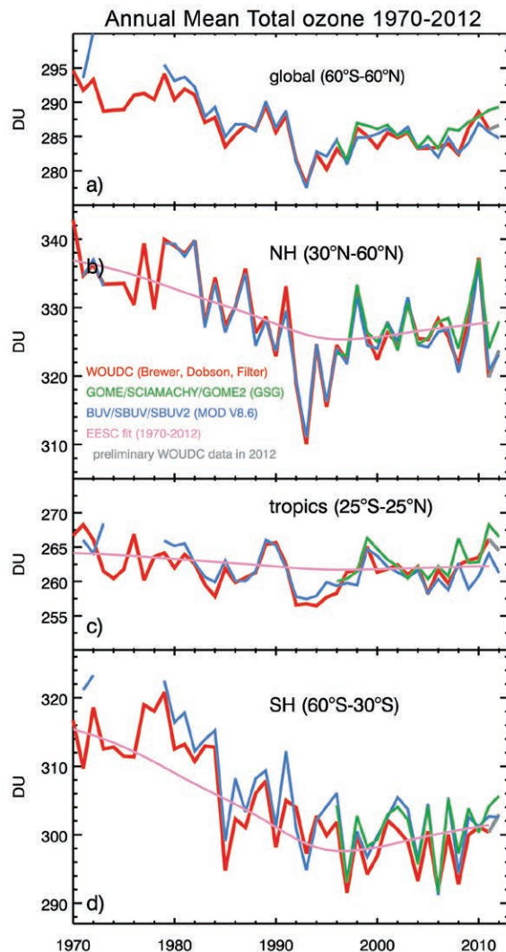
FIG. 2.36. Annual mean total ozone (DU) from measurements combining ground-based Brewer, Dobson, and filter spectrometer data (red; Fioletov et al. 2002, 2008), BUUV/SBUV MOD V8.6 (blue; Stolarski and Frith 2006), and GOME/SCIAMACHY/GOME-2 “GSG” (green; Weber et al. 2007), in the (a) 60°N–60°S (global), (b) 30°N–60°N (NH), (c) 25°N–25°S (tropics), and (d) 30°S–60°S (SH) zonal bands. Annual mean in 2012 from the ground-based data does not include December data and is considered preliminary as all 2012 station data were not available as of this publication date. The smooth magenta curves show long-term ozone response to changes in stratospheric halogens.
