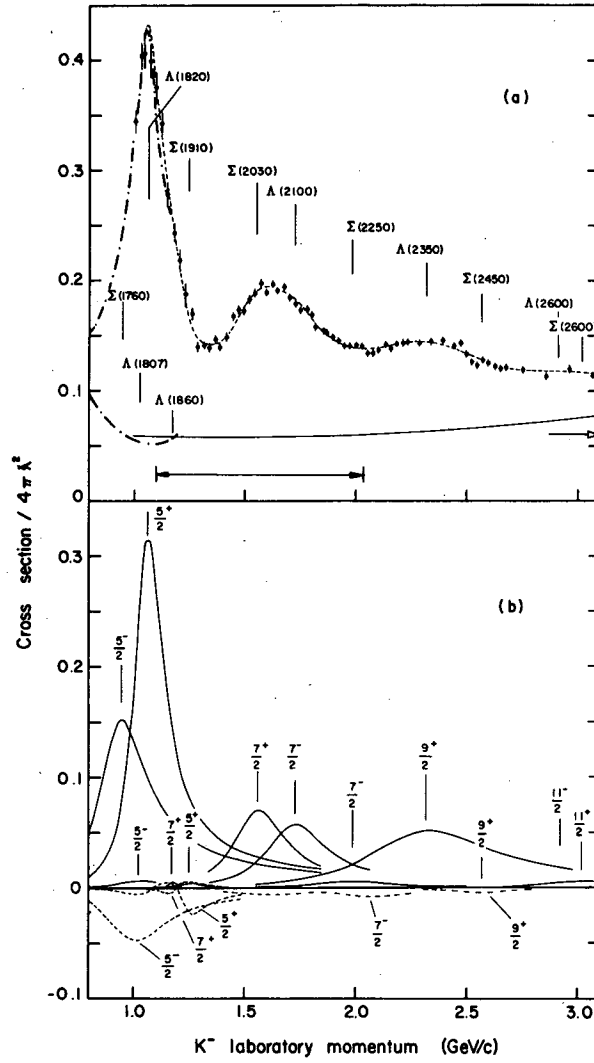
FIG. 5(a). Cross section divided by 4\pi\lambda^2 versus incident K^- momentum for the reaction K^-p \rightarrow \bar{K}^0n as measured by Bricman et al. 10 The dashed curve is the result of their fit, the solid line is the contribution of the background, and the vertical lines indicate the position of the resonances included in the fit. (b) The solid lines represent the contribution of the resonances to the fitted curve, the dashed lines represent the interference terms for each partial wave.
