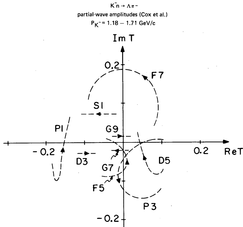
FIG. 8. Partial-wave amplitudes for the reaction K^-n \rightarrow \Lambda\pi^- obtained by Cox et al. 16 (rotated by 180 deg so as to agree with our sign convention). Arrows indicate the direction of increasing energy.
