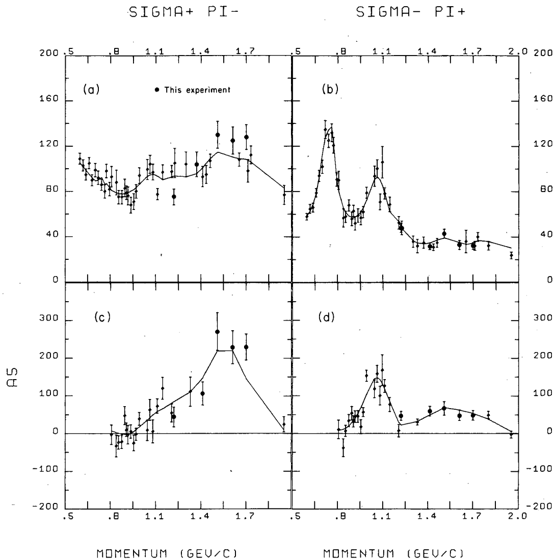
FIG. 13. Some data for the reaction K^-p \rightarrow \Sigma\pi . (a) and (b) The A_0 = \sigma/4\pi\lambda^2 coefficients for the \Sigma^+\pi^- and \Sigma^-\pi^+ channel respectively. (c) and (d) The A_5 coefficients for the same two channels. Data are from Refs. 21, 15, and 20. The curves are the result of fit C discussed in the text.
