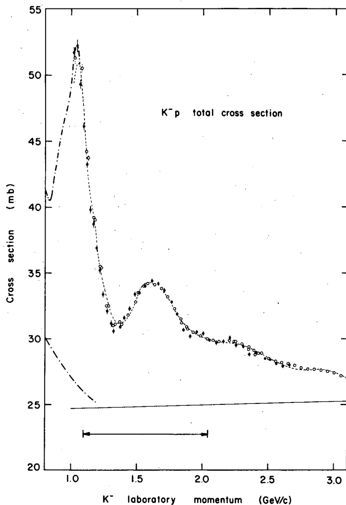
FIG. 4. Compilation of the total K^-p cross section data, 8 taken from Bricman et al. 10 The dashed line is their fit to the data, the solid line is the contribution from the assumed linear background. The horizontal line shows the region of interest in this paper.
