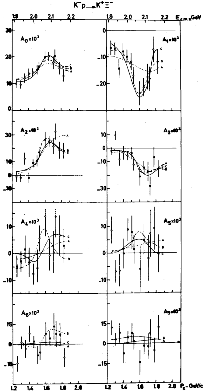
FIG. 16. The coefficients of the differential cross section for the reaction K^-p \rightarrow K^+\Xi^- reported by Burgun et al. 22 The curves correspond to the three fits discussed in the text.
