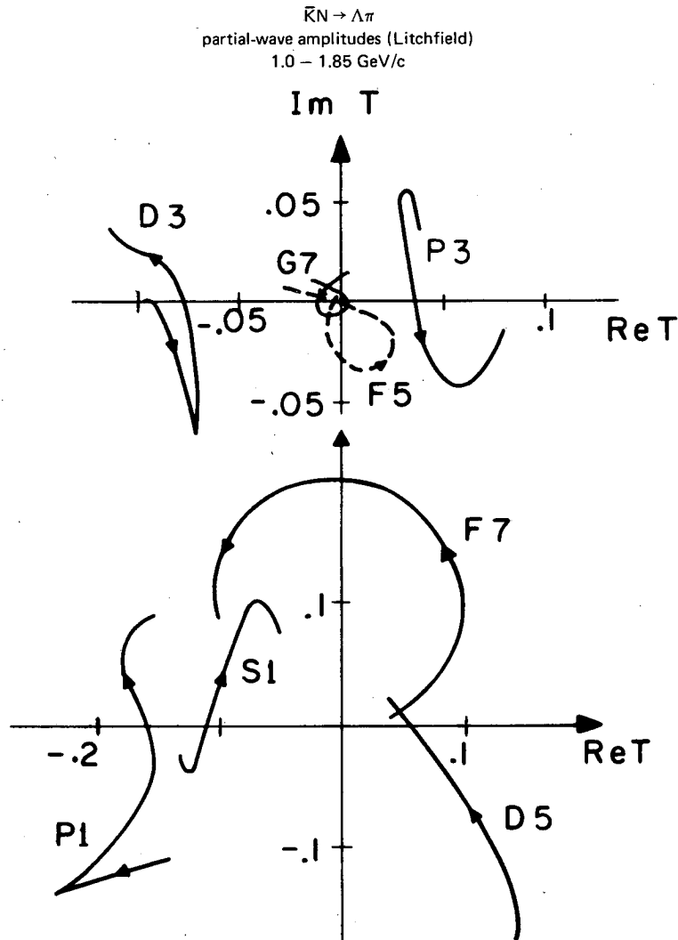
FIG. 9. Partial-wave amplitudes for the \Lambda\pi channel, result of the analysis of Litchfield. 17 Only fit A is shown, fit B being very similar. Litchfield used all the data included in the three previous analyses.
