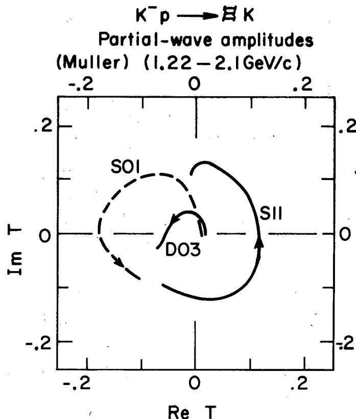
FIG. 17. Some partial-wave amplitudes for the reaction K^-N \rightarrow \Xi K as found by Muller 23 , using a u-channel exchange parameterization. The energy range shown here is from 1.22 to 2.1 GeV/c.
