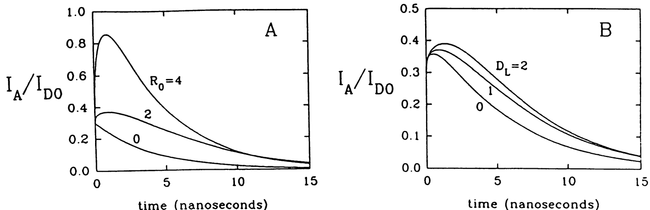
FIGURE 14 Translational motion only. The acceptor intensity over the initial donor intensity versus the time after the flash in example 3, for N = the number of states = 10, k_D = the inverse of the donor radiative decay rate = 1/6 \text{ ns}^{-1} , s = the shortest donor-acceptor distance (occurring in state 1) = 1 nm, a = the medium donor-acceptor distance = 3 nm, \sigma = the width of the Gaussian distribution = 0.5 nm, \epsilon = I_{A0}/I_{D0} has been set equal to 0.3 ( \epsilon is the ratio of acceptor absorbance over donor absorbance at donor excitation wavelengths). (A) D_L = the lateral diffusion constant (defined in the text) = 1 \text{ nm}^2/\text{ns} , R_0 = the Förster distance = 0, 2, 4 nm; (B) R_0 = 2 \text{ nm} , D_L = 0, 1, 2 \text{ nm}^2/\text{ns} .
