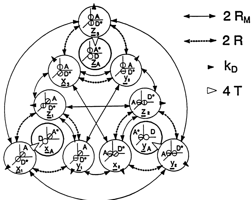
FIGURE 5 Rotational motion only in an isotropic system. The excited donor states of example 2 (labeled with D^* ), x_i , y_i , and z_i ( i = 1, 2, 3 ) are shown with their donor and acceptor moments (lines in the dumbbells). The transitions between these states are also indicated. These are due to molecular rotations at a rate R_M and intermolecular donor rotations at a rate R . The nonradiative decay at a rate k_D as well as transfer are denoted. The rate of transfer to excited acceptor states (also shown, labeled with A^* ), z_A , x_A , or y_A , is nonzero only for the transitions x_1 to x_A , y_2 to y_A , and z_3 to z_A , and this rate constant is equal to 4T . The direction of the acceptor transition moments of the excited acceptor states are also shown.
