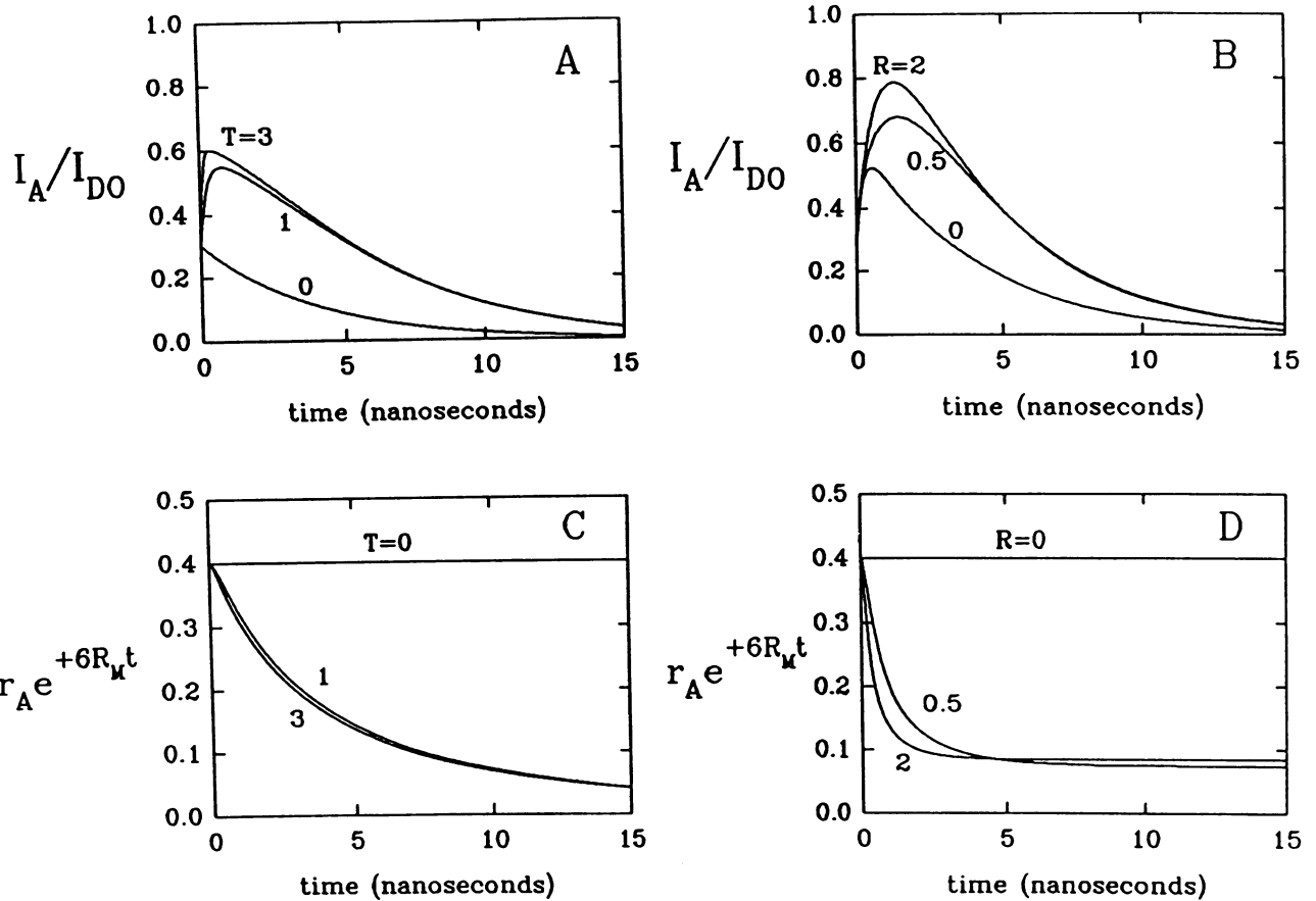
FIGURE 9 Rotational motion only in an isotropic system. The dependence of the time-resolved acceptor fluorescence and anisotropy on the rate of transfer and rotation is shown for example 2. T is the rate of transfer from the donor to the acceptor at unit orientation factor, k_D^{-1} = 6 ns ( k_D is the rate of radiative decay of the donor), k_A^{-1} = 4 ns ( k_A is the rate of radiative decay of the acceptor), and \epsilon = I_{A0}/I_{D0} = 0.3 ( \epsilon is the ratio of acceptor absorbance over donor absorbance at donor excitation wavelengths). Here R and R_M represent rotational rate constants. Compare with Fig. 10, where R and R_M denote rotational diffusion constants, and the size of the cutoff matrices is 11 \times 11 (see Appendix D). (A) Intensity; (C) anisotropy with R = 0.1 ns ^{-1} , T = 0, 1 , and 3 ns ^{-1} . (B) Intensity; (D) anisotropy with R = 0, 0.5 , and 2 ns ^{-1} , T = 1 ns ^{-1} . The anisotropy does not depend on R_M except for a factor \exp(-6R_M t) . The anisotropy divided by this factor is plotted in Figs. 9, C and D and 10, C and D.
