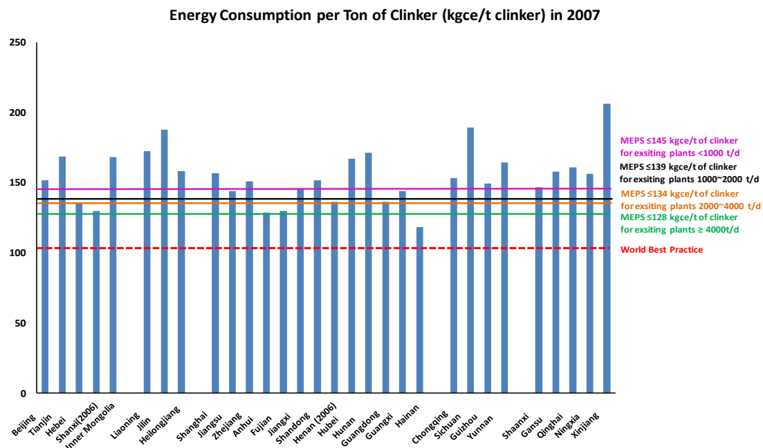
Figure 20. Benchmarking of Energy Intensity of the Cement Clinker Production in China 48
