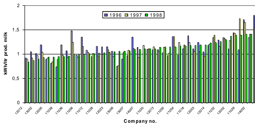
Figure 10 Comparison of Electricity Use per Liter of Milk Produced for IEEN Companies, 1996-1998.
