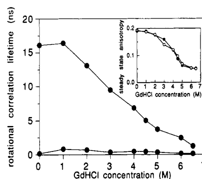
FIGURE 4: Rotational correlation times of holo-HSOD measured as a function of GdHCl concentration. Inset: experimental (filled symbols) and calculated (open symbols) steady-state fluorescence anisotropy of holo-HSOD as a function of GdHCl concentration. The steady-state anisotropy was calculated on the basis of the dynamic anisotropy values shown in the main panel.
