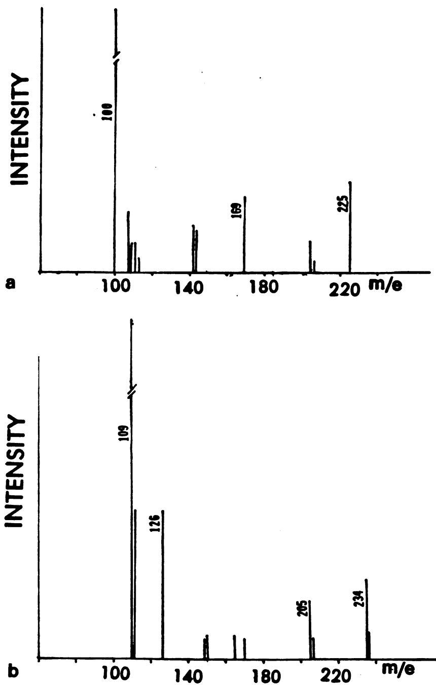
Figure 24. Mass spectra obtained from (a) lyophilized reaction mixture after 5 hours incubation of CCNU with phosphate buffer, pH 7.4, 37°C (b) pure CCNU.
