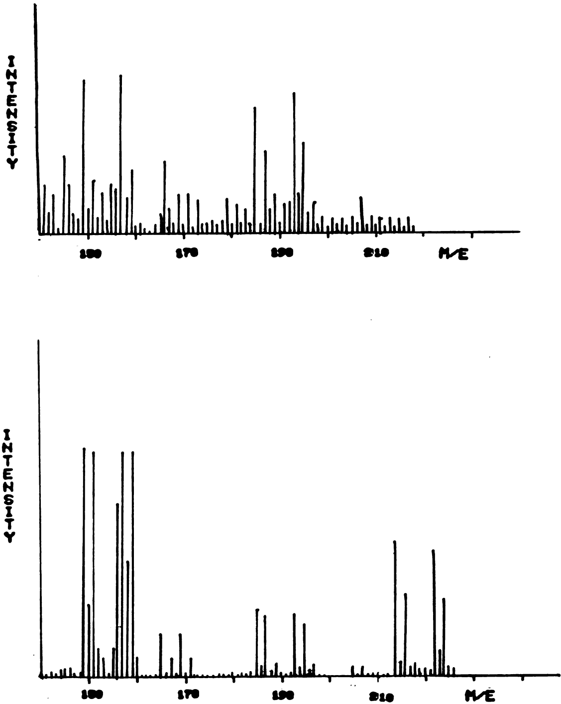
Figure 33. Mass spectra of BCU formed in vitro metabolism by rat liver microsomes (upper) and unreacted BCNU, both were collected from HPLC column.
