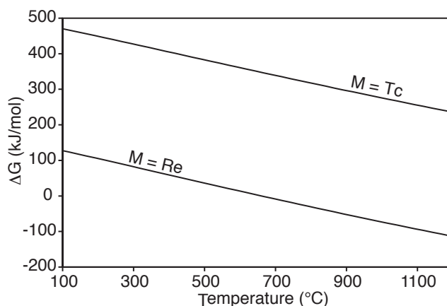
Figure 6. Plot of the Gibbs free energy of reaction 5 as a function of temperature. Disproportionation of Re(IV) becomes exothermic at high temperature.
