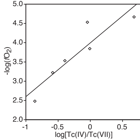
Figure 5. Relationship of Tc redox state to oxygen fugacity determined from Fe(II)/ΣFe. Data are indicated by diamonds and the least-squares fit is indicated by the solid line.
