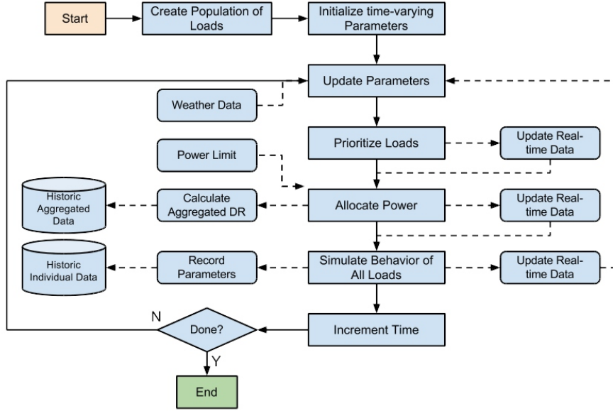
Figure 7: Proposed algorithm for aggregation of flexible loads
