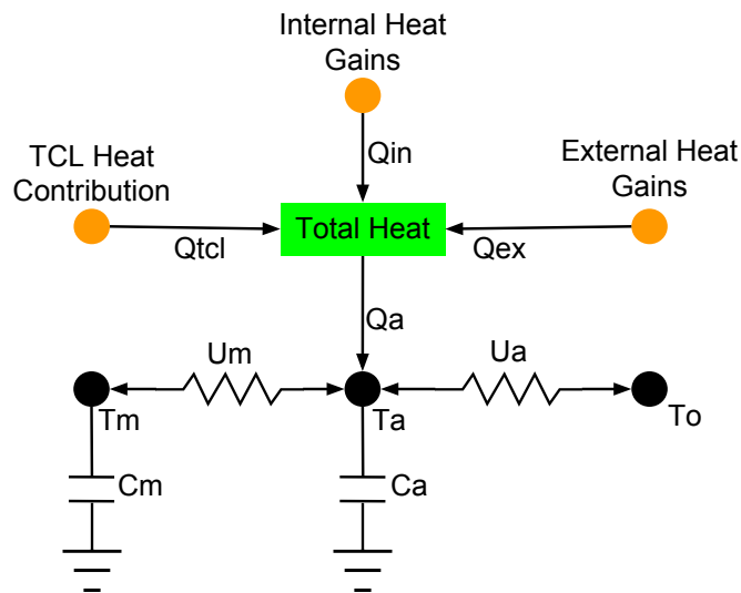
Figure 2: Representation of Equivalent Thermal Parameter (ETP) model
