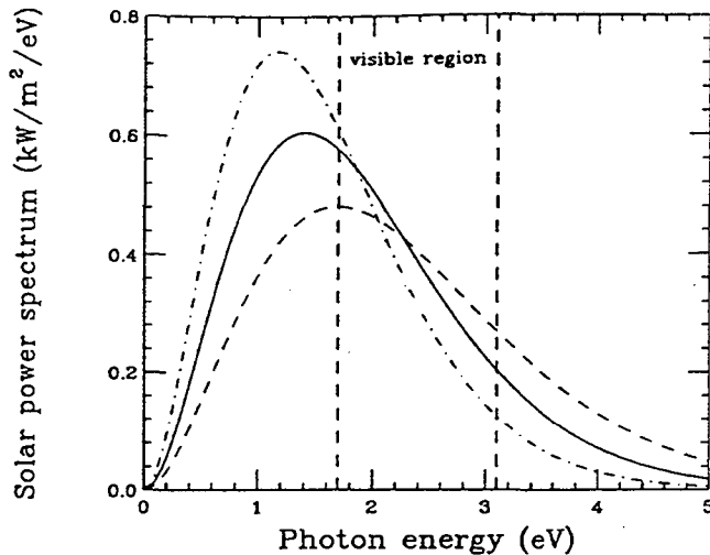
FIG. 2. Solar power spectrum incident on the Earth ( \text{kW}/\text{m}^2/\text{eV} ). Solid curve, actual spectrum, surface temperature 5800 K. Dot-dashed curve, W mass one-half of actual value, giving a surface temperature 4800 K, a luminosity 1.025 times actual, and a radius 1.45 times actual. Dashed curve, W mass twice actual value, giving a surface temperature 7000 K, a luminosity 0.96 times actual, and a radius 0.67 times the actual radius. The visible region from 1.7 eV ( \lambda=792 nm) to 3.1 eV ( \lambda=400 nm) is indicated. The calculations and curves were provided by J. D. Jackson (Jackson, 1995).
