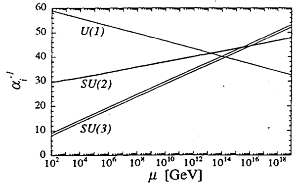
FIG. 3. The evolution of the couplings of the standard model without supersymmetry. The electromagnetic and weak couplings are combinations of U(1) and SU(2) . The strong coupling is denoted SU(3) . If the interactions arise from a single grand unified force, the three couplings should come together at a single point. The figure was provided by H. Murayama.
