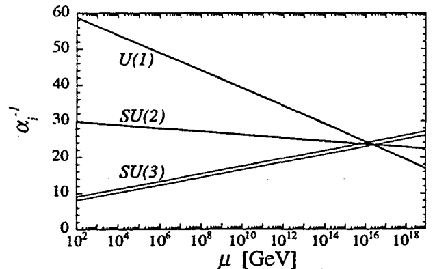
FIG. 4. The evolution of the couplings of the standard model with supersymmetry. Because the supersymmetric world has extra particles, the evolution of the couplings is different than in the non-supersymmetric world. In the supersymmetric model the couplings converge at a single point, suggesting there is unification of the electroweak and strong interactions. The figure was provided by H. Murayama.
