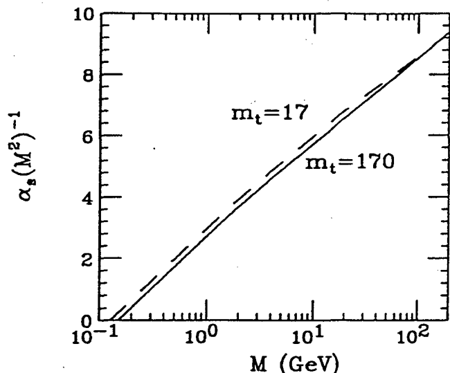
FIG. 1. The evolution of the reciprocal of the strong coupling, \alpha_s(M^2)^{-1} , as a function of the mass scale, M^2 , shown both for our world ( m_t = 170 GeV, solid line) and an alternative world ( m_t = 17 GeV, dashed line). The alternative world has smaller values of the coupling and thus smaller values of the parameter \Lambda . In the alternative world, the proton would be lighter by a factor 0.84.
