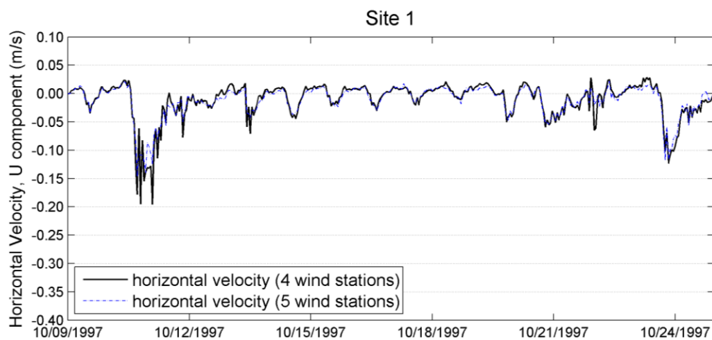
Figure 13. East/West velocity components for wind fields test
