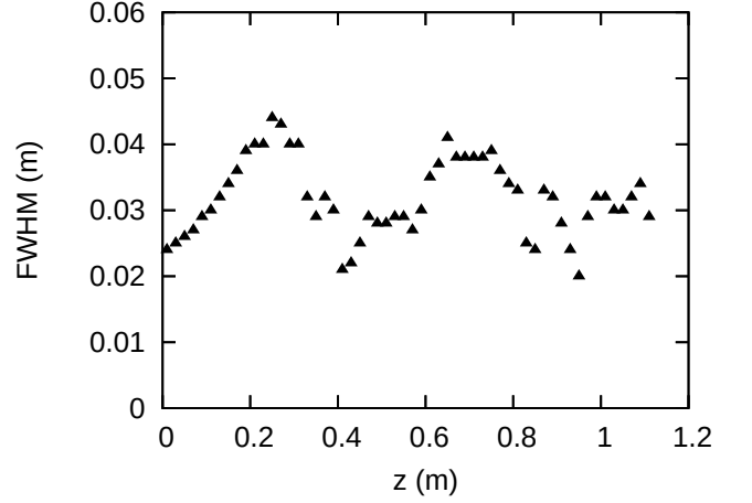
FIG. 2: Evolution of the pulse FWHM. The data marked by triangles are for the same guided simulation parameters as used in Fig. 1. The initial spot size was r_0 = 2.0 cm.
