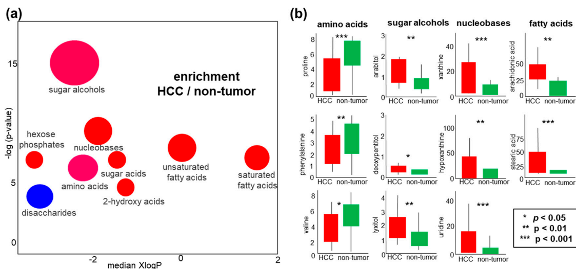
Figure 4. Differential regulation of liver metabolites in HCC tumors versus non-malignant tissues. (a) Chemical set enrichment statistics of significantly regulated metabolites. Colors of chemical sets: red = increased, blue = decreased, purple = sets with compounds decreased and increased. Ball sizes represent the number of compounds per metabolic set. XlogP represents the median lipophilicity of the metabolic clusters. (b) Examples of boxplots (medians and interquartile ranges) of individual compounds that showed univariate significant differences. Units of all y-axes: normalized peak intensities in 10,000 ion counts/spectrum for each quantification ion (Supplementary S1).
