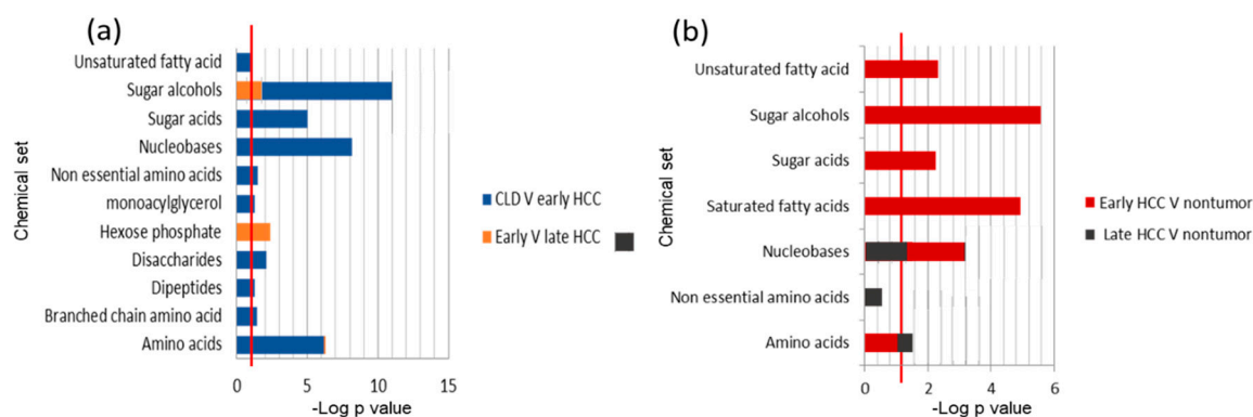
Figure 7. ChemRICH set enrichment statistics comparison for blood (a) and HCC tissues metabolites (b). (a) Significant chemical sets in blood metabolites for early HCC patients versus CLD subjects (blue) and comparing early-stage HCC versus late-stage HCC (orange). (b) Significant chemical sets in HCC tumor metabolites to paired non-malignant liver tissues for early HCC stages (red) and late HCC stages (black). The set enrichment significance level of p < 0.05 ( -\log p = 1.3 ) is indicated by red lines.
