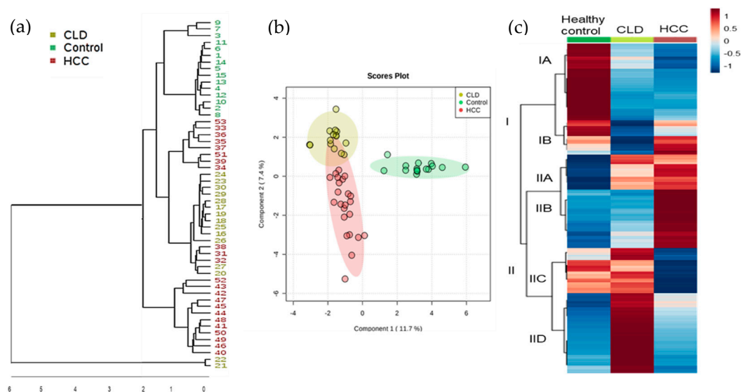
Figure 1. Multivariate clustering of blood-based metabolomics data using GC-TOF mass spectrometry. (a) Unsupervised hierarchical clustering of all 730 detected metabolites in the studied groups HCC, Chronic Liver Disease (CLD), and healthy control. (b) Supervised sparse partial least squares-discriminant analysis of all 730 metabolites to better distinguish metabolotypes of study groups. (c) Clustering of 510 significant metabolites (Mann–Whitney U test p < 0.05 and qFDR < 0.1 ) across the three test groups, range-scaled from increased (+1, red) to decreased (−1, blue).
