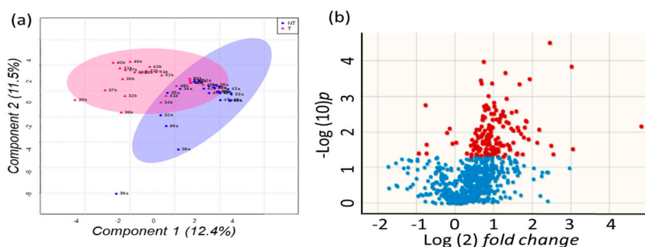
Figure 3. Multivariate analysis of 730 peaks detected by untargeted GC-TOF MS metabolomics analysis of paired HCC tumors versus non-malignant liver tissues. (a) sparse Projections to Latent Structures Discriminant Analysis (sPLS-DA). Blue: non-malignant tissues, red: tumor biopsies. Percentages give the total explained variance for vectors 1 and 2. (b) Volcano plot for differential regulation of metabolites. Blue: not significant at raw p < 0.05 , red: significant changes at p < 0.05 .
