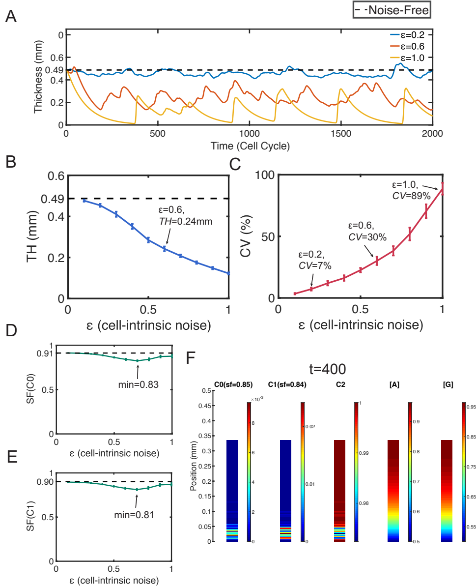
Figure 3. Simulations with only cell-intrinsic noise. Dash lines represent the corresponding quantities at homeostasis. A. Layer thickness in three simulations with \epsilon = 0.2, 0.6 and 1 . B. The mean TH . The error bars show the standard deviation. C. The mean CV . The error bars show the standard deviation of CV . The mean SF of D. stem cells and E. TA cells. The error bars show the standard deviation. F. Distribution of cells and morphogens in a specific simulation with \epsilon = 0.6 at time t = 400 . In (B-E) , all statistical quantities are captured based on 20 simulations, and the standard deviations (error bars) are negligible compared to the means.
