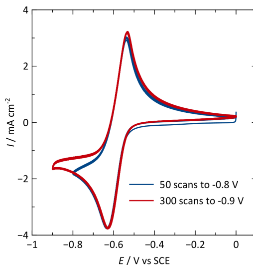
Figure 29. Extended cyclic voltammetry of MV/Br electrolyte. Repeated cyclic voltammograms of 50 mM \text{MVCl}_2 /0.2 M KBr electrolyte are shown for 50 scans to -0.8 V followed by 300 scans to -0.9 V at a scan rate of 10 mV/s.
