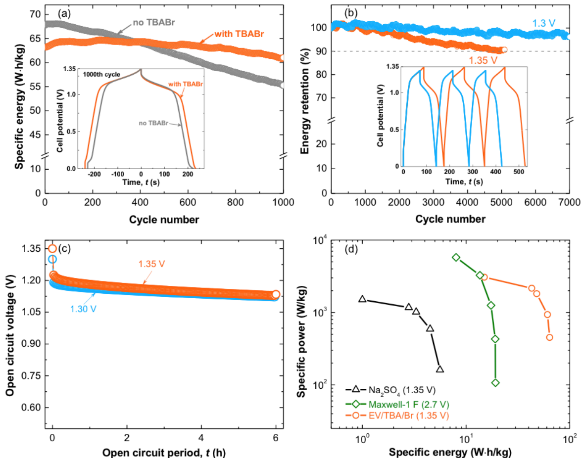
Figure 48. A 1.2 M EVBr 2 /0.12 M TBABr/2.88 M NaBr cell. (a) Specific energy and cycling stability of EV/Br cells with and without TBABr; the inset shows GCD profiles at the 1000 th cycle. (b) Long-term cycling stability of the EV/TBA/Br cell cycled at 2 A/g to 1.3 V, and to 1.35 V; the inset shows GCD profiles for the last 3 cycles. (c) Open circuit voltage for 6 h after charging the cell to 1.35 V (orange curve) and 1.3 V (blue curve), respectively. (d) Specific energy vs power of the EV/TBA/Br cell (orange curve) and its comparison to Na 2 SO 4 (black curve) and commercial Maxwell (green curve) cells. Specific energy and power of all cells, including the commercial EDLC, were normalized to the dry mass of both positive and negative electrodes. Rate tests of the EV/TBA/Br cell were performed after the initial 1000 GCD cycles at 1 A/g.
