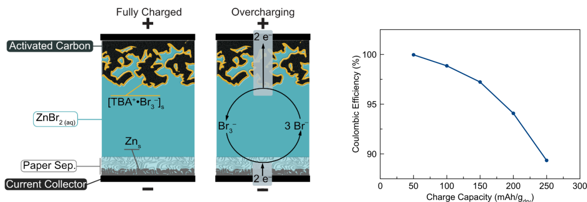
Figure 60. Built-in self-balancing mechanism to prevent overcharging of ZnBr 2 cells. (schematic) Overcharging the ZnBr 2 chemistry causes uncomplexed tribromide to diffuse across the cell, which creates a temporary internal short circuit. This redox shuttle mechanism can prevent overcharging damage to individual cells and help balance multiple cells when they are connected in series. Note that the electrolyte volume is exaggerated in the schematic. In actual cells, the activated carbon electrode touches the separator and electrolyte only resides in the porous separator and electrode. (plot) Coulombic efficiency versus charging capacity – a ZnBr 2 /TBABr pouch cell was cycled at 1 A/g to different capacity limits in 50 mAh/g increments. Coulombic efficiency decreases substantially when the cell is overcharged, due to a finite quantity of TBABr complexing agent.
