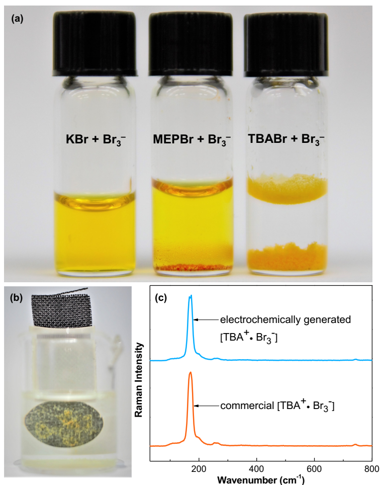
Figure 40. Complexation of tribromide with different quaternary ammonium species. (a) Complexation of chemically generated Br 3 - by the addition of potassium bromide (left), MEPBr (middle), and TBABr (right). (b) Electrochemically generated [TBA + · Br 3 - ] solid complex by controlled potential electrolysis. (c) Raman spectra of the electrochemically generated [TBA + · Br 3 - ] solid complex (blue curve) and commercial [TBA + · Br 3 - ] solid complex (orange curve).
