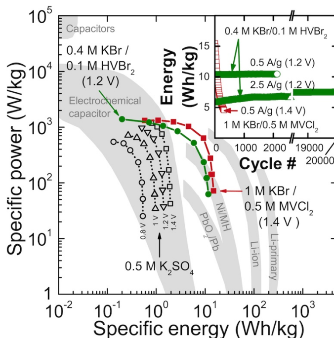
Figure 21. Ragone plot of redox EC performance from volume-limiting cells.
