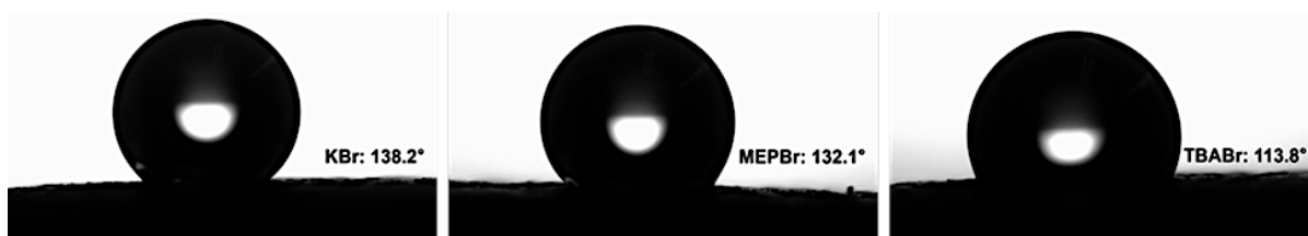
Figure 38. Contact angle of test electrolyte on the surface of a porous activated carbon pellet. (left) aqueous KBr solution droplet; (middle) aqueous MEPBr solution droplet; (right) aqueous TBABr solution droplet.
