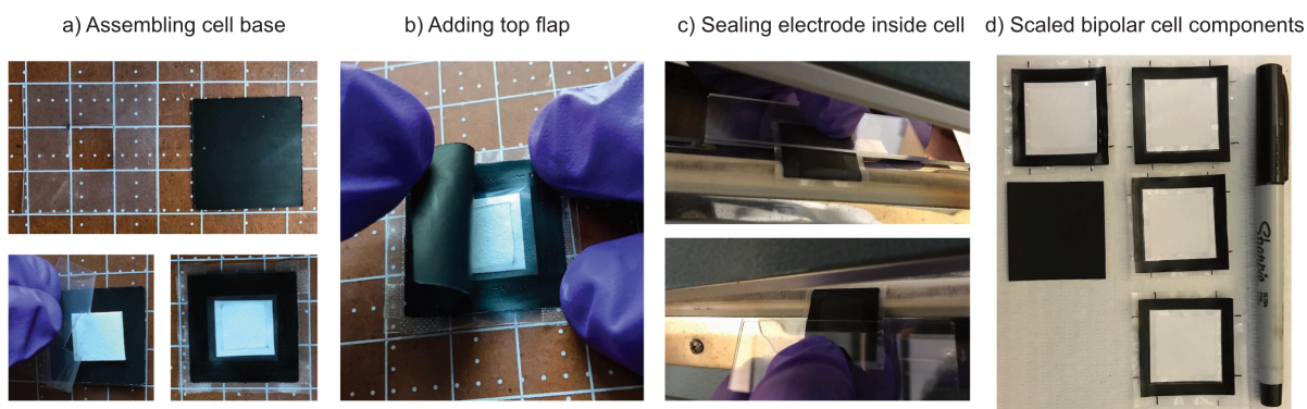
Figure 50. Assembly of pouch cells. (a) The plastic spacer is heat-sealed to all four edges of the negative CBPE CC. (b) The positive CBPE CC is heat-sealed to the other side of the plastic spacer on one edge to create a flexible flap. (c) After adding \text{ZnBr}_2 electrolyte and the positive electrode, the flap is closed and the remaining three edges are sealed. (d) Current collectors prepared for the scaled bipolar pouch before assembly. A negative CC/plastic spacer assembly (top left), positive CC (middle left), and three bipolar CC/plastic spacer assemblies (right) are shown. The markings on the plastic spacers are to assist with alignment.
