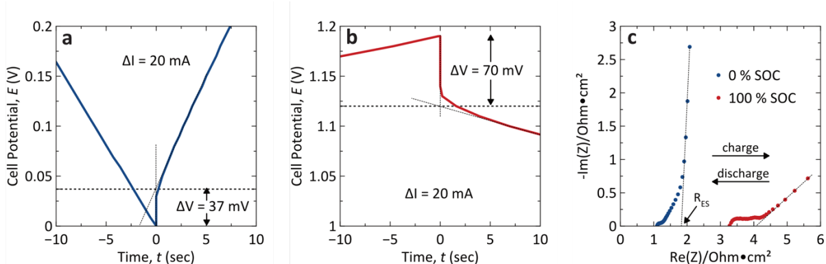
Figure 36. Measuring equivalent series resistance ( R_{ES} ). IR drop for a 1 M \text{PVBr}_2/3 M NaBr cell immediately after (a) discharging and (b) charging at \pm 10 mA, as well as (c) Nyquist impedance spectra from 0.2 MHz to 0.1 Hz for the fully discharged (0 % SOC) and fully charged (100 % SOC) conditions. The increase in R_{ES} in the charged state is evidenced by the larger IR drop, contact resistance, and charge transfer resistance. This behavior is related to the formation of precipitated solid complexes with low electrical conductivity at both electrodes, and consistent with the operating mechanism of the cell.
