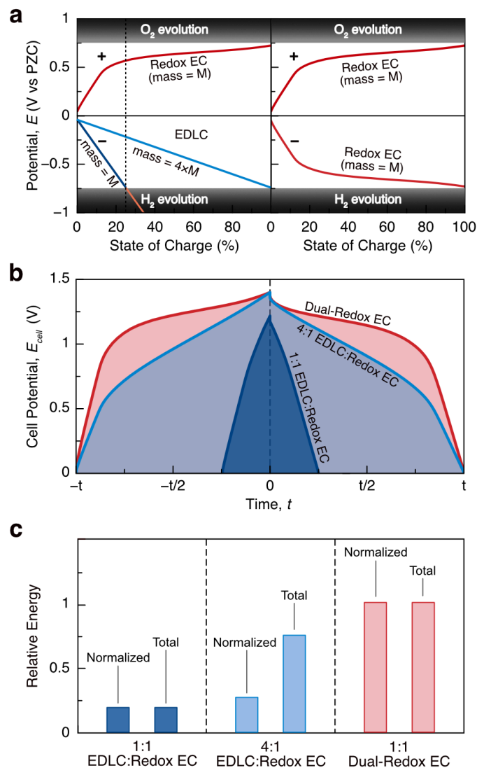
Figure 5. Balancing the capacity of a redox EC electrode. (a) Galvanostatic charging potential profiles for a redox EC electrode with an EDLC counter electrode of equal mass, an EDLC counter electrode with four times higher mass, or another redox EC electrode of equal mass (dual-redox EC). (b) The energy stored by each combination is proportional to the area under the resulting full-cell potential profiles. (c) The relative total and normalized (gravimetric or volumetric) energy stored by systems with an EDLC counter electrode is much less than the dual-redox EC configuration.
