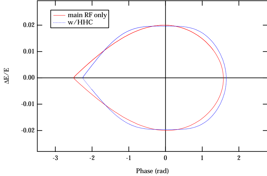
FIG. 3. RF bucket with and without harmonic voltage and optimum flattening. The RF acceptance is reduced slightly with the harmonic voltage reducing the lifetime increase from the bunch lengthening.
