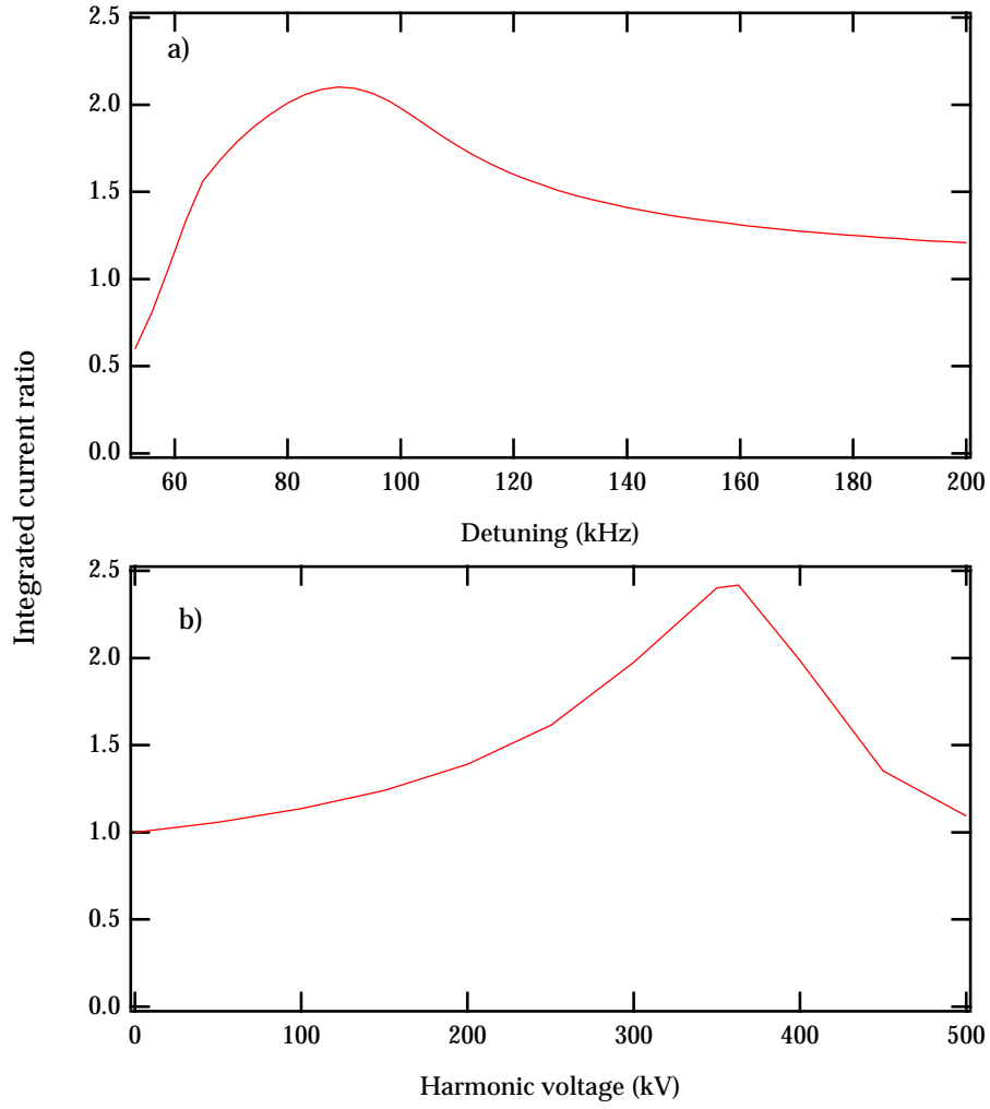
FIG. 9. Increase in integrated current for an SC cavity with a) fixed detuning and b) fixed voltage.
