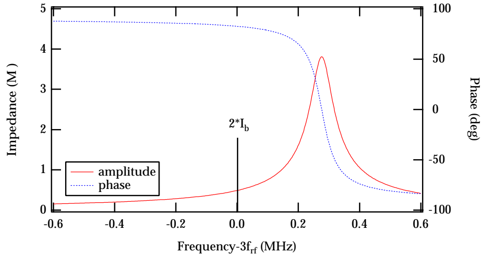
FIG. 4. Tuning of the fundamental mode of the harmonic cavity for reaching optimum bunch lengthening voltage and phase.
