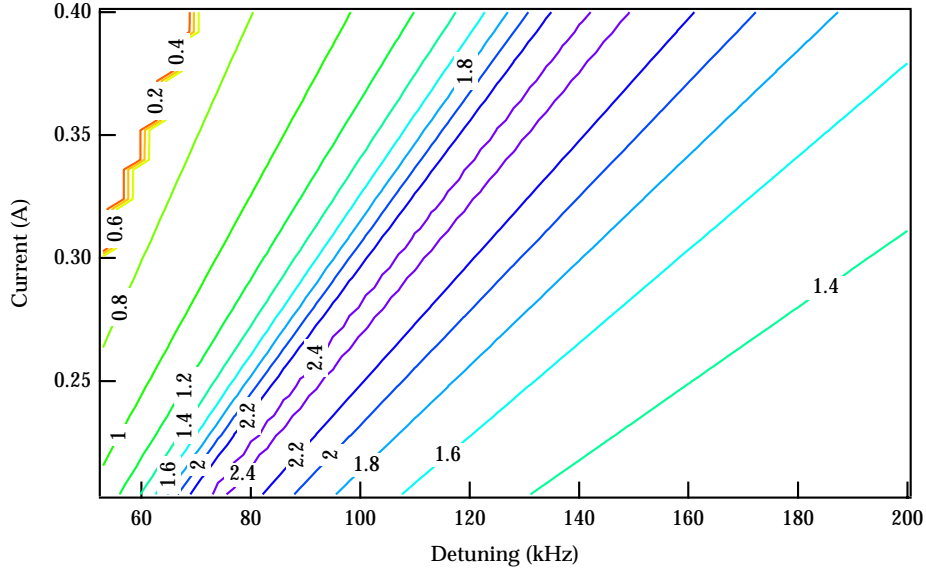
FIG. 8. Contour plot of the relative lifetime improvement as a function of beam current and detuning for 1 SC cavity.
