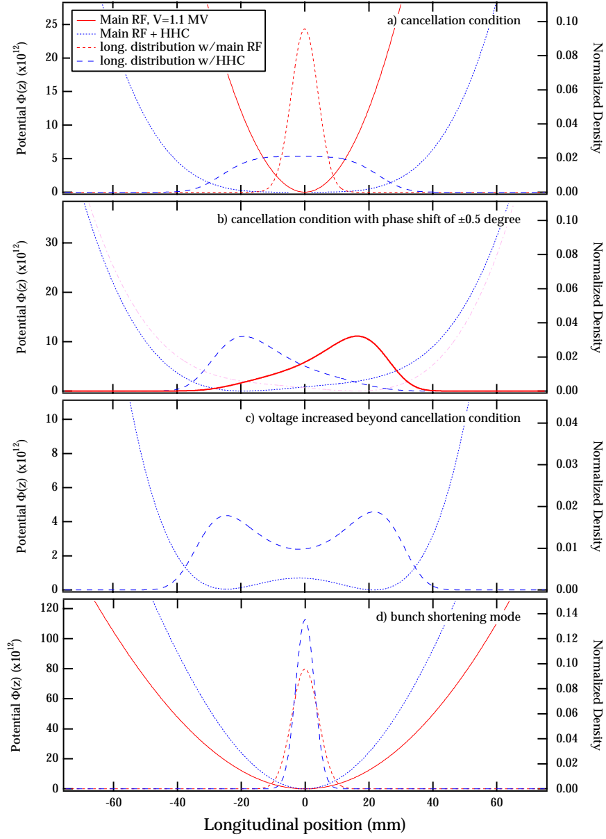
FIG. 2. Potential well and longitudinal distribution for several cases of harmonic voltage.
