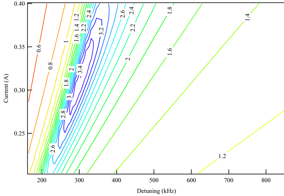
FIG. 5. Contour plot of the relative lifetime improvement as a function of beam current and detuning for 3 NC cavities for ALS 1.9 GeV conditions.
