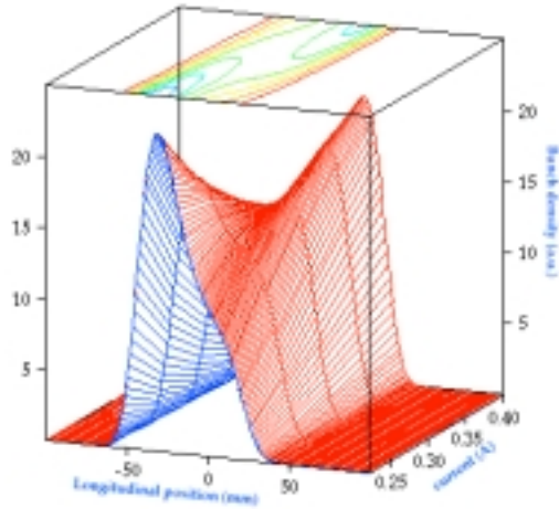
FIG. 7. Top) Evolution of the bunch shape over a fill for the case of a fixed detuning at 330 kHz. The bunch shape and phase change much less than for the case of a constant voltage but with a lower increase in integrated current. Bottom) Fixed voltage of 360 kV. The bunch phase slips forward and behind the synchronous phase above and below the current where the maximum bunch length occurs.
