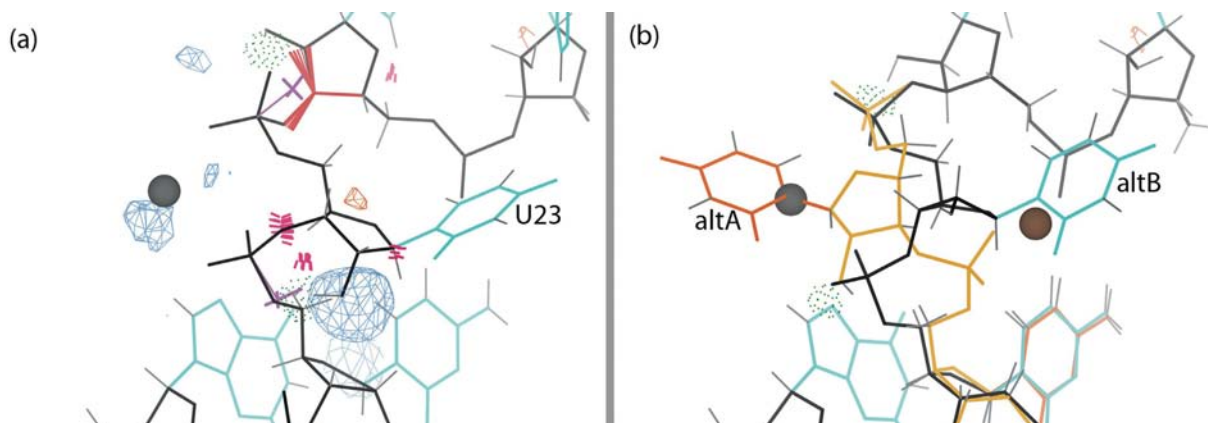
Figure 3. U23 and Mg^{2+} of the cleaved structure with Fo-Fc difference density at 3.5\sigma contour level. Here and in later figures, the blue and orange mesh correspond to positive and negative difference density respectively, hydrogen bonds are shown as green dotted pillows, steric clashes as hotpink spikes, ribose pucker outliers as magenta crosses, and bond-length or bond-angle outliers as springs or fans (blue if too small, red if too large). (a) The base and backbone of U23 in the original structure (1CX0), with the modeling errors highlighted. (b) Alternate conformations of U23 in the rebuilt structure (4PR6), with the backbone (gold), base (orange) and metal ion (brown) for the new conformation. All the modeling errors are corrected, and the difference density peaks have disappeared.
