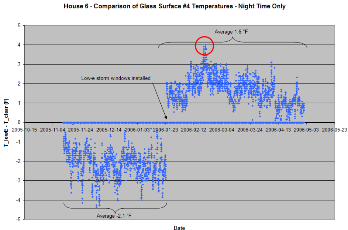
Figure 2 – Interior glass surface temperature differences at the room side (#4) for side-by-side windows having no storm windows (prior to 1/23/2006) and after one was fitted with a low-e storm window and the other with a clear glass storm window, as a function of time.
