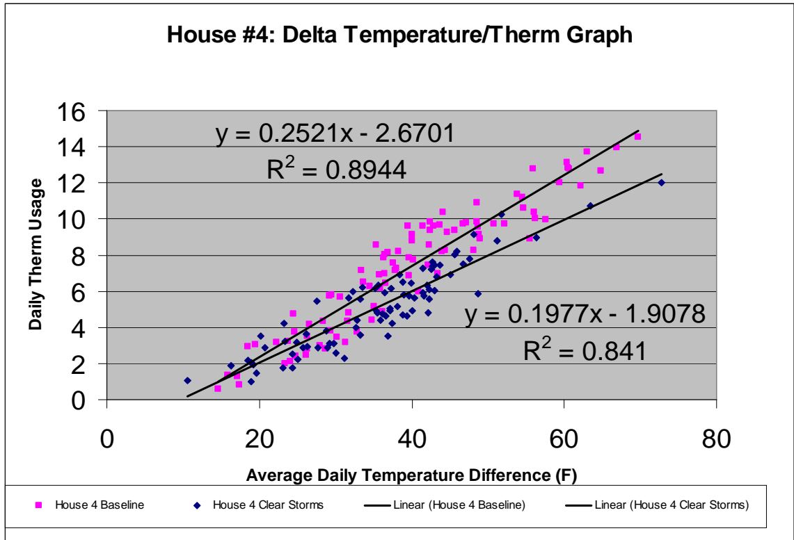
Figure 1: House #4: Delta Temperature/ Daily Therm Usage Graph
