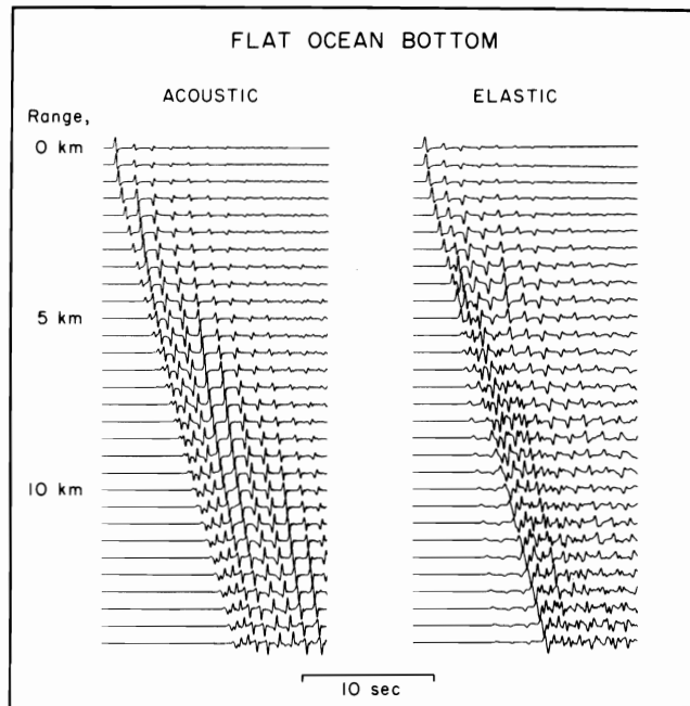
Figure 6. The results for acoustic and elastic simulations in the model shown in Figure 5 without the ridge. The results show the importance of including elastic coupling in the sea floor.
