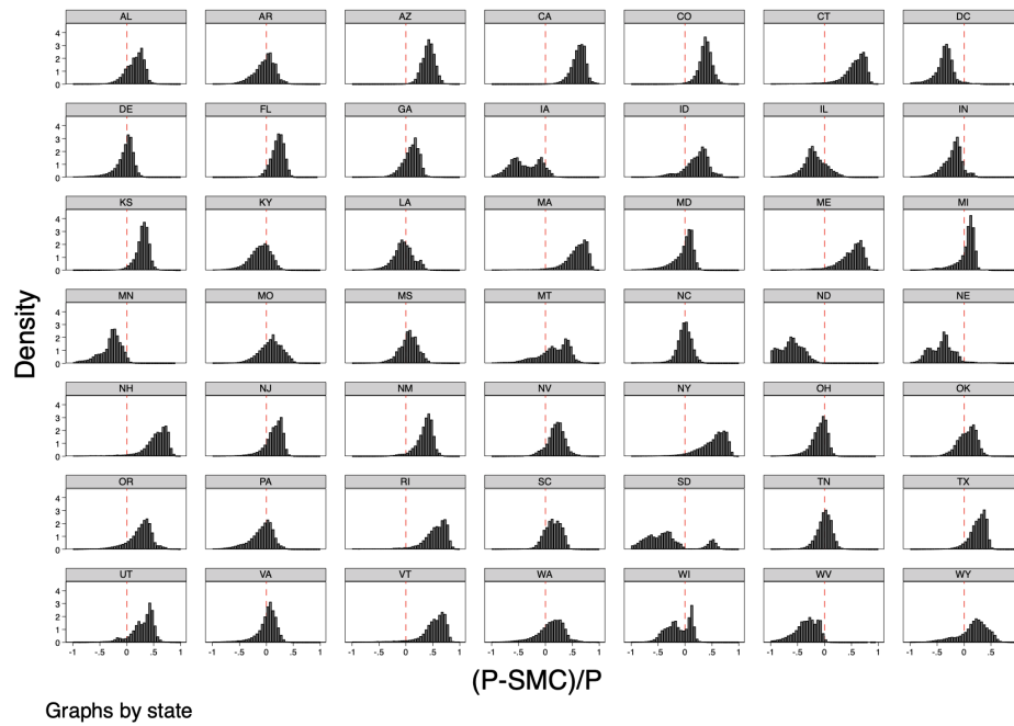
Figure 10: Hourly Price Markup ( \frac{P-SMC}{P} ) by State
