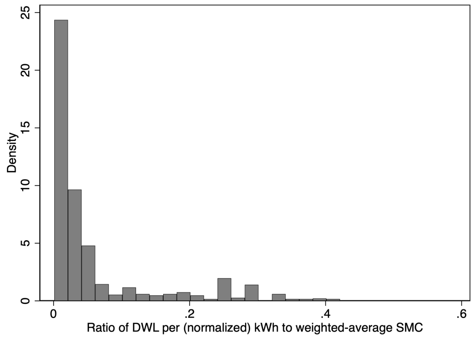
Figure 12: Distribution of DWL/SMC Ratio
